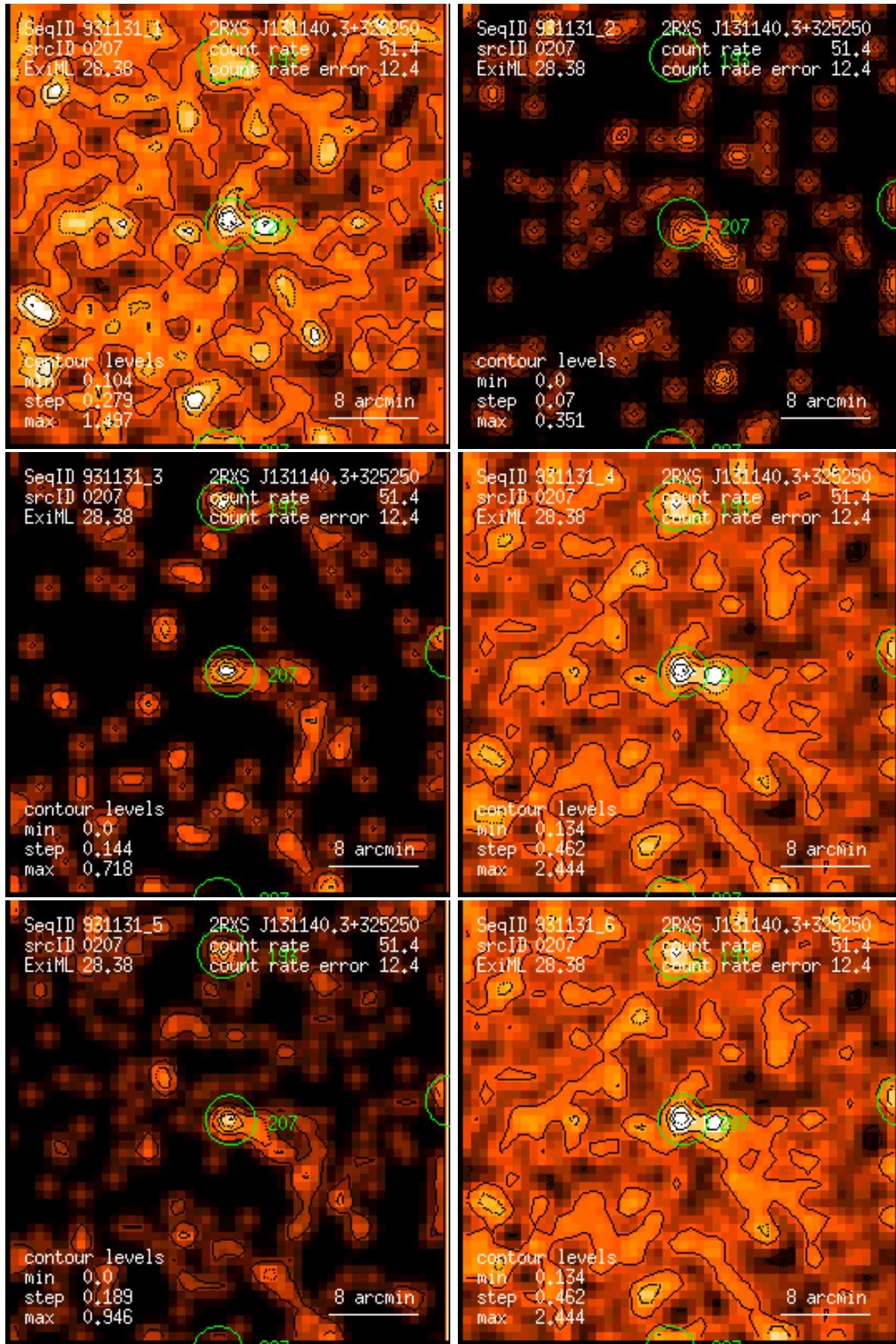
Figure 207: RASS 931131: detection 0207: band rate images, Gaussian filter: (1) PSPC channels 11 – 41, (2) 52 – 90, (3) 91 – 201, (4) 11 – 235, (5) 52 – 201, (6) 11 – 201. Broad band rates in counts/ks. Band rate contour levels in counts/ks/arcmin 2 .
