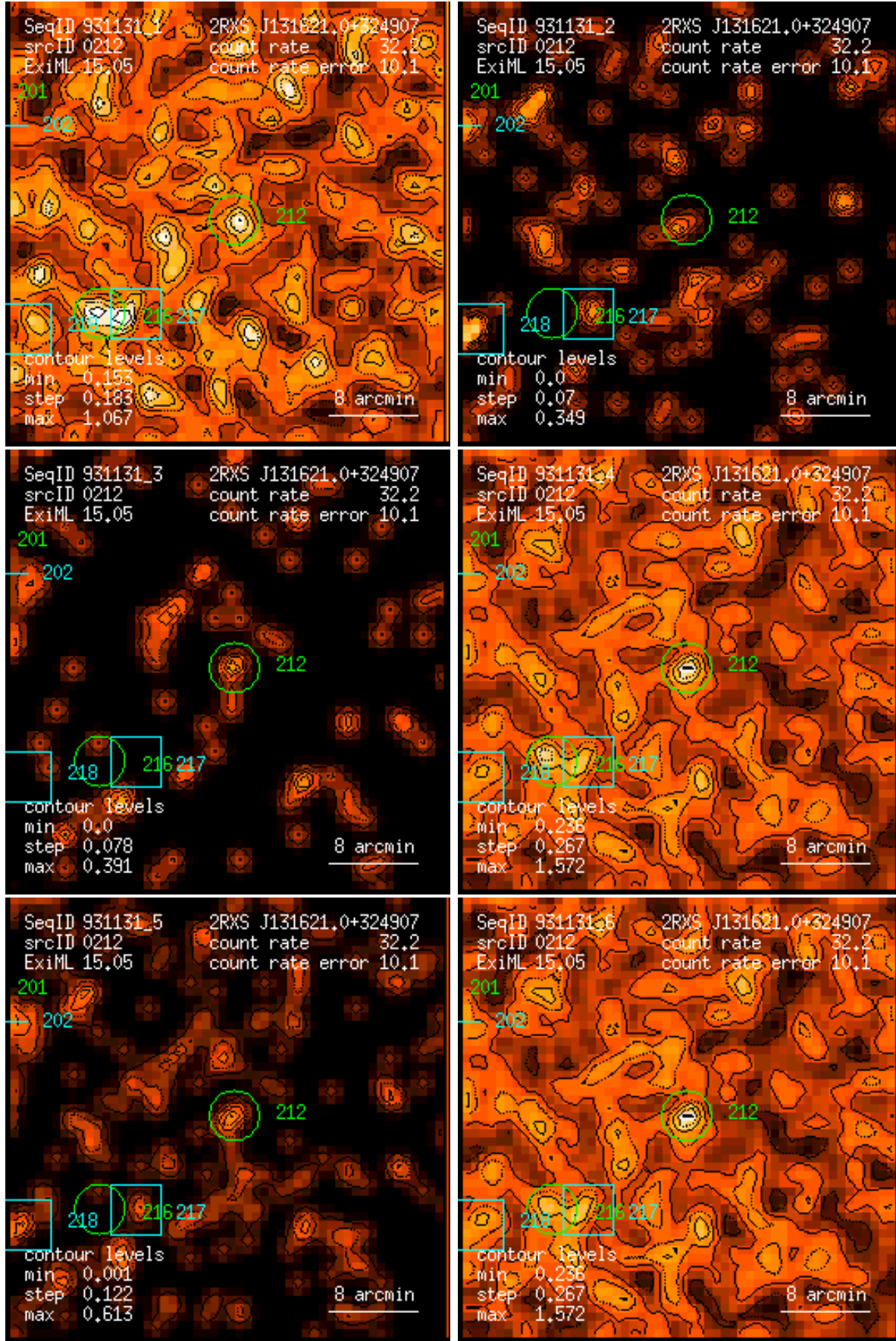
Figure 212: RASS 931131: detection 0212: band rate images, Gaussian filter: (1) PSPC channels 11 – 41, (2) 52 – 90, (3) 91 – 201, (4) 11 – 235, (5) 52 – 201, (6) 11 – 201. Broad band rates in counts/ks. Band rate contour levels in counts/ks/arcmin 2 .
