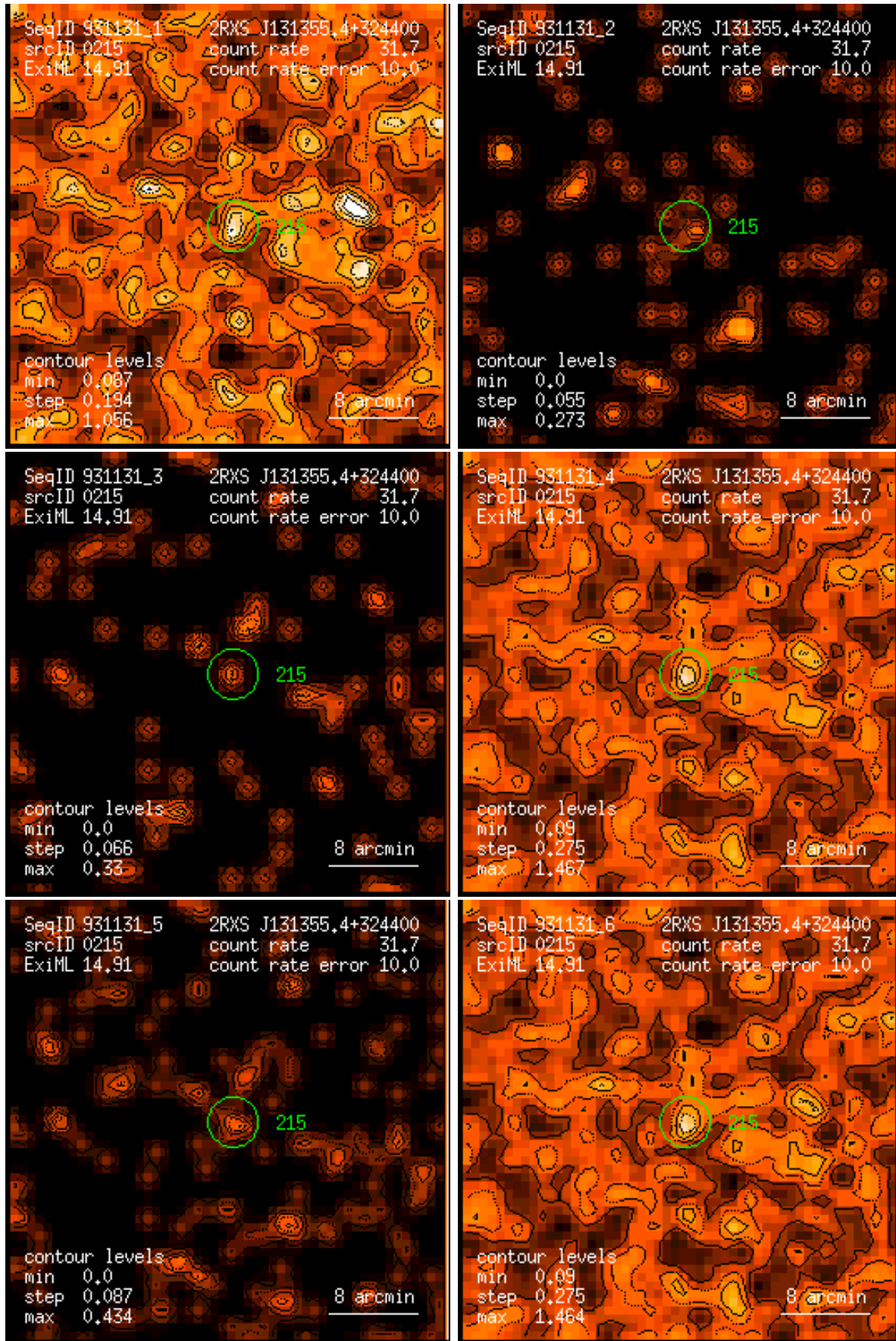
Figure 215: RASS 931131: detection 0215: band rate images, Gaussian filter: (1) PSPC channels 11 – 41, (2) 52 – 90, (3) 91 – 201, (4) 11 – 235, (5) 52 – 201, (6) 11 – 201. Broad band rates in counts/ks. Band rate contour levels in counts/ks/arcmin 2 .
