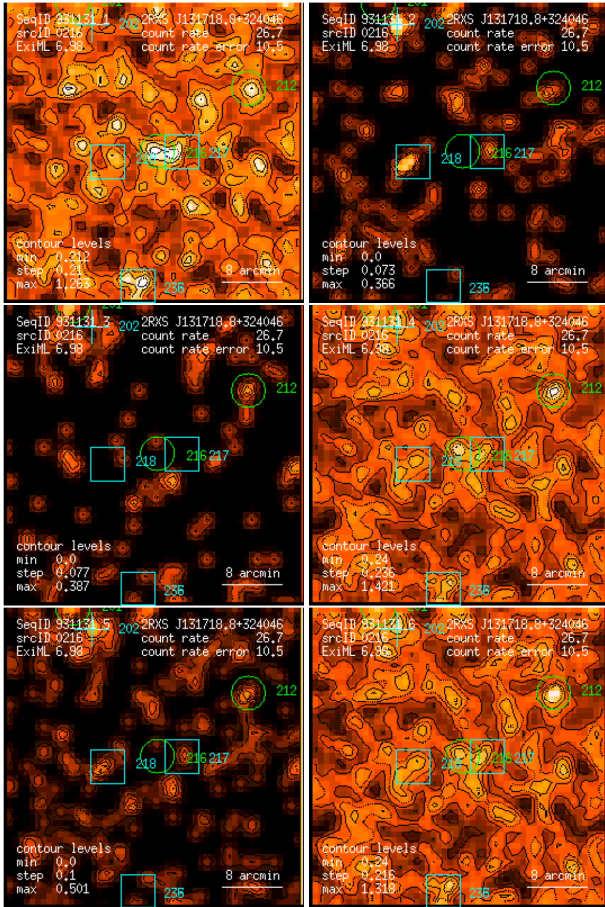
Figure 216: RASS 931131: detection 0216: band rate images, Gaussian filter: (1) PSPC channels 11 – 41, (2) 52 – 90, (3) 91 – 201, (4) 11 – 235, (5) 52 – 201, (6) 11 – 201. Broad band rates in counts/ks. Band rate contour levels in counts/ks/arcmin 2 .
