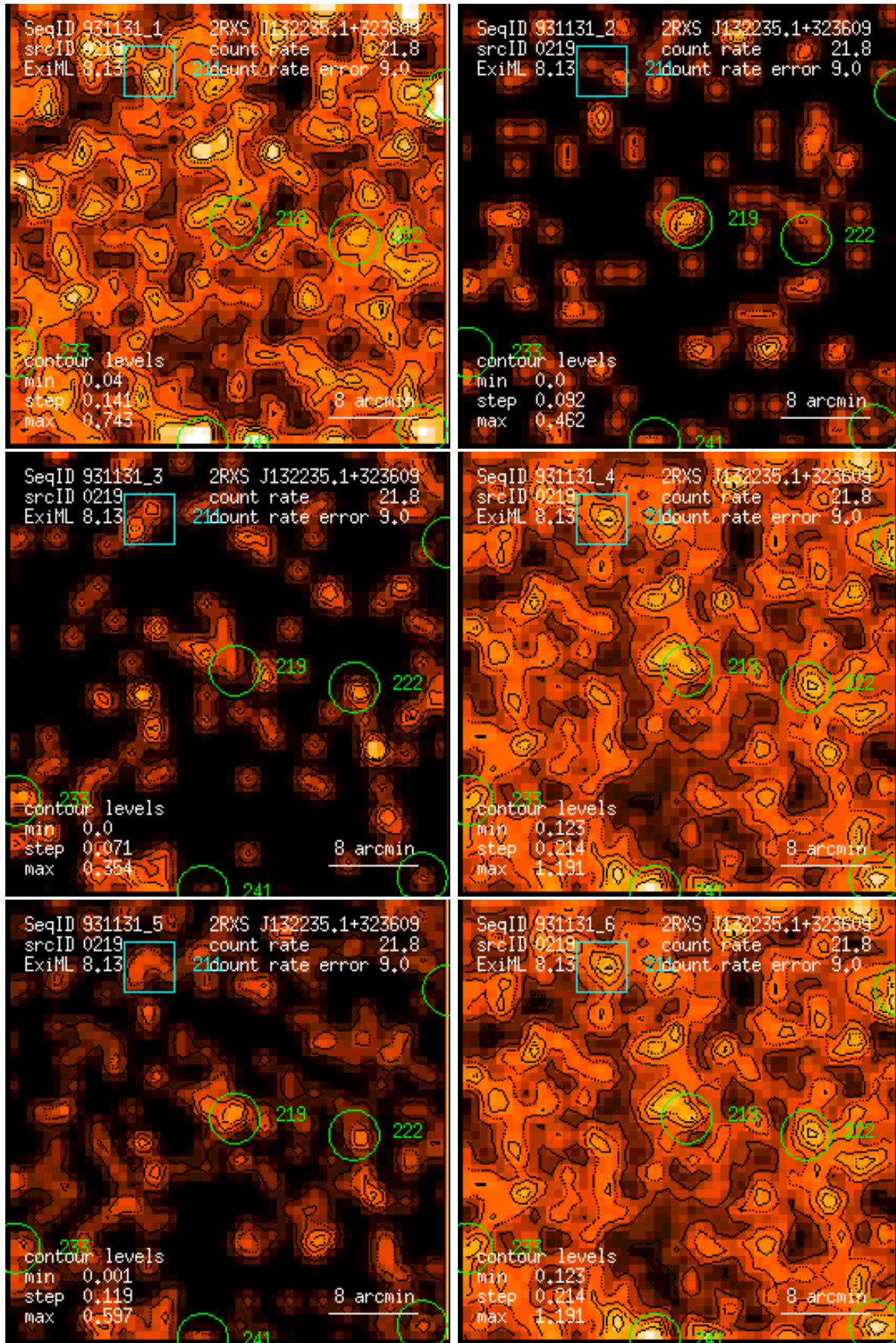
Figure 219: RASS 931131: detection 0219: band rate images, Gaussian filter: (1) PSPC channels 11 – 41, (2) 52 – 90, (3) 91 – 201, (4) 11 – 235, (5) 52 – 201, (6) 11 – 201. Broad band rates in counts/ks. Band rate contour levels in counts/ks/arcmin 2 .
