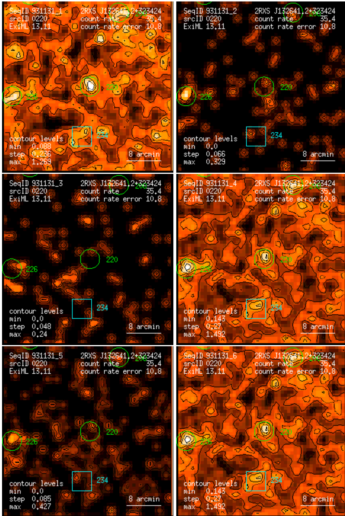
Figure 220: RASS 931131: detection 0220: band rate images, Gaussian filter: (1) PSPC channels 11 – 41, (2) 52 – 90, (3) 91 – 201, (4) 11 – 235, (5) 52 – 201, (6) 11 – 201. Broad band rates in counts/ks. Band rate contour levels in counts/ks/arcmin 2 .
