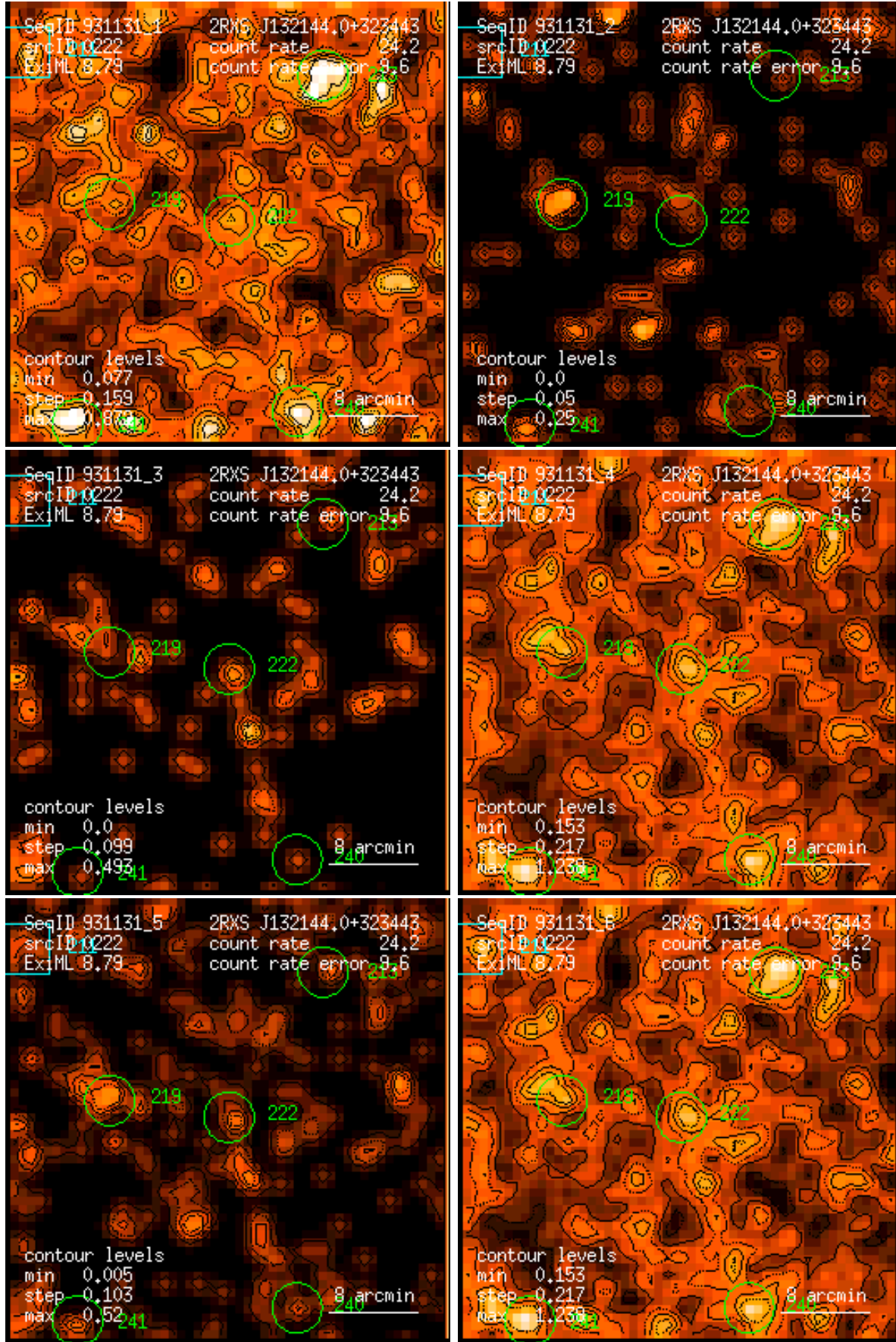
Figure 222: RASS 931131: detection 0222: band rate images, Gaussian filter: (1) PSPC channels 11 – 41, (2) 52 – 90, (3) 91 – 201, (4) 11 – 235, (5) 52 – 201, (6) 11 – 201. Broad band rates in counts/ks. Band rate contour levels in counts/ks/arcmin 2 .
