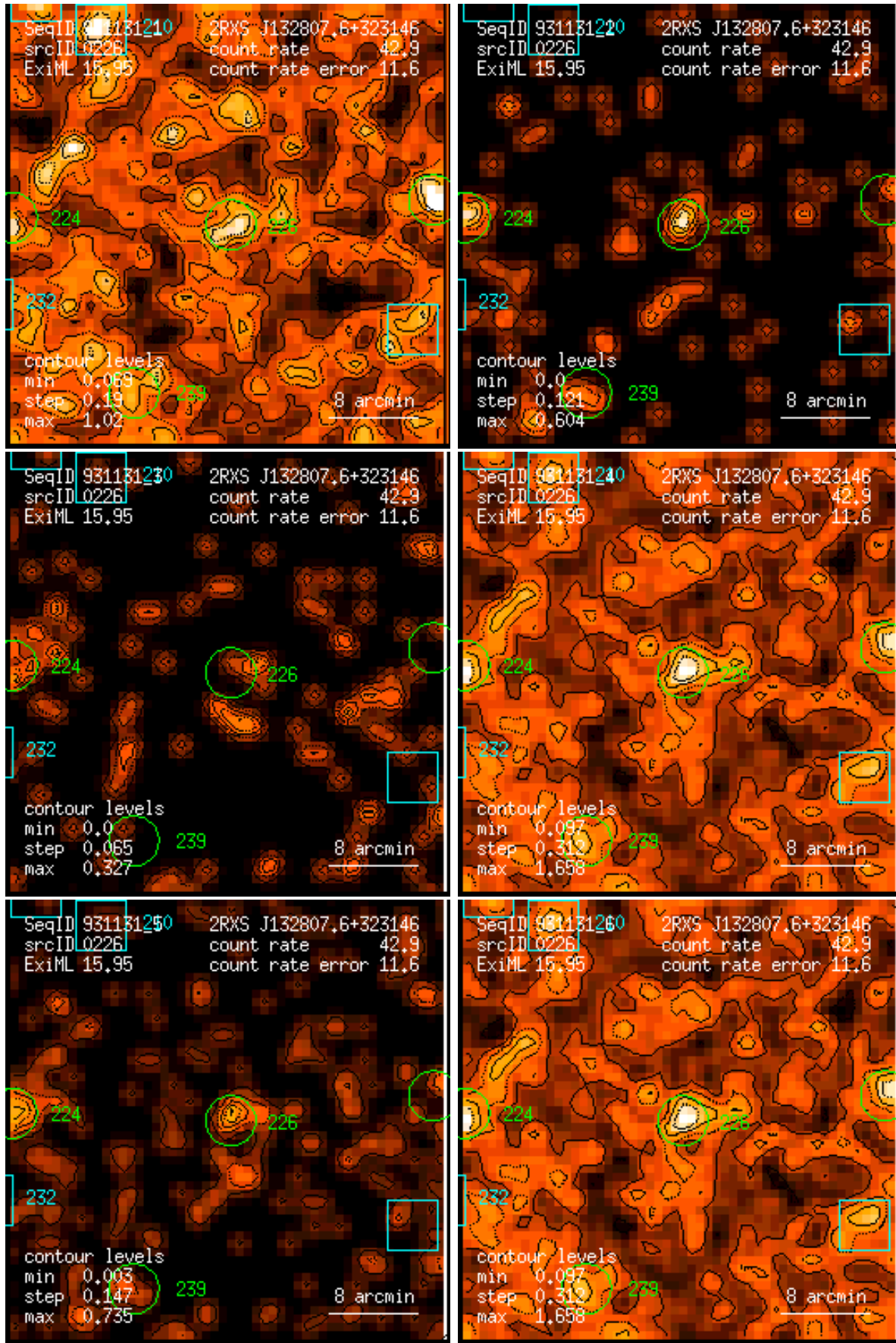
Figure 226: RASS 931131: detection 0226: band rate images, Gaussian filter: (1) PSPC channels 11 – 41, (2) 52 – 90, (3) 91 – 201, (4) 11 – 235, (5) 52 – 201, (6) 11 – 201. Broad band rates in counts/ks. Band rate contour levels in counts/ks/arcmin 2 .
