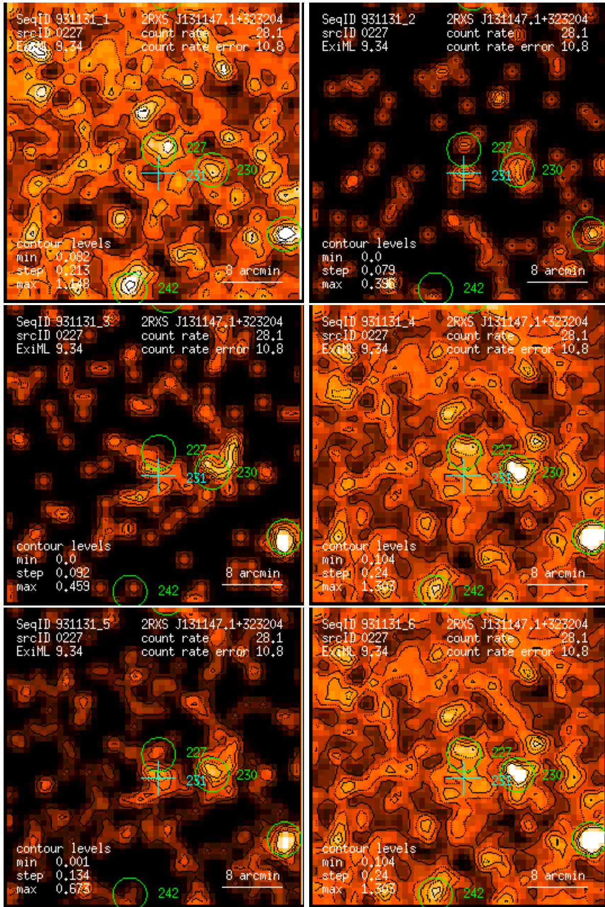
Figure 227: RASS 931131: detection 0227: band rate images, Gaussian filter: (1) PSPC channels 11 – 41, (2) 52 – 90, (3) 91 – 201, (4) 11 – 235, (5) 52 – 201, (6) 11 – 201. Broad band rates in counts/ks. Band rate contour levels in counts/ks/arcmin 2 .
