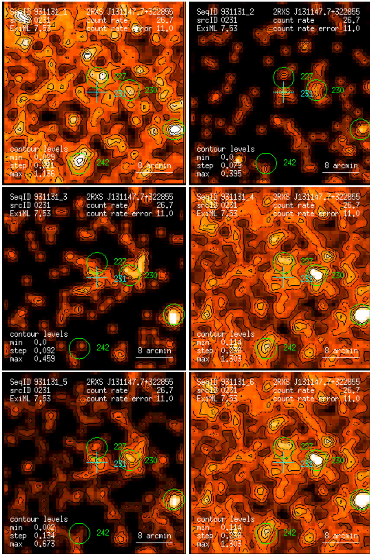
Figure 231: RASS 931131: detection 0231: band rate images, Gaussian filter: (1) PSPC channels 11 – 41, (2) 52 – 90, (3) 91 – 201, (4) 11 – 235, (5) 52 – 201, (6) 11 – 201. Broad band rates in counts/ks. Band rate contour levels in counts/ks/arcmin 2 .
