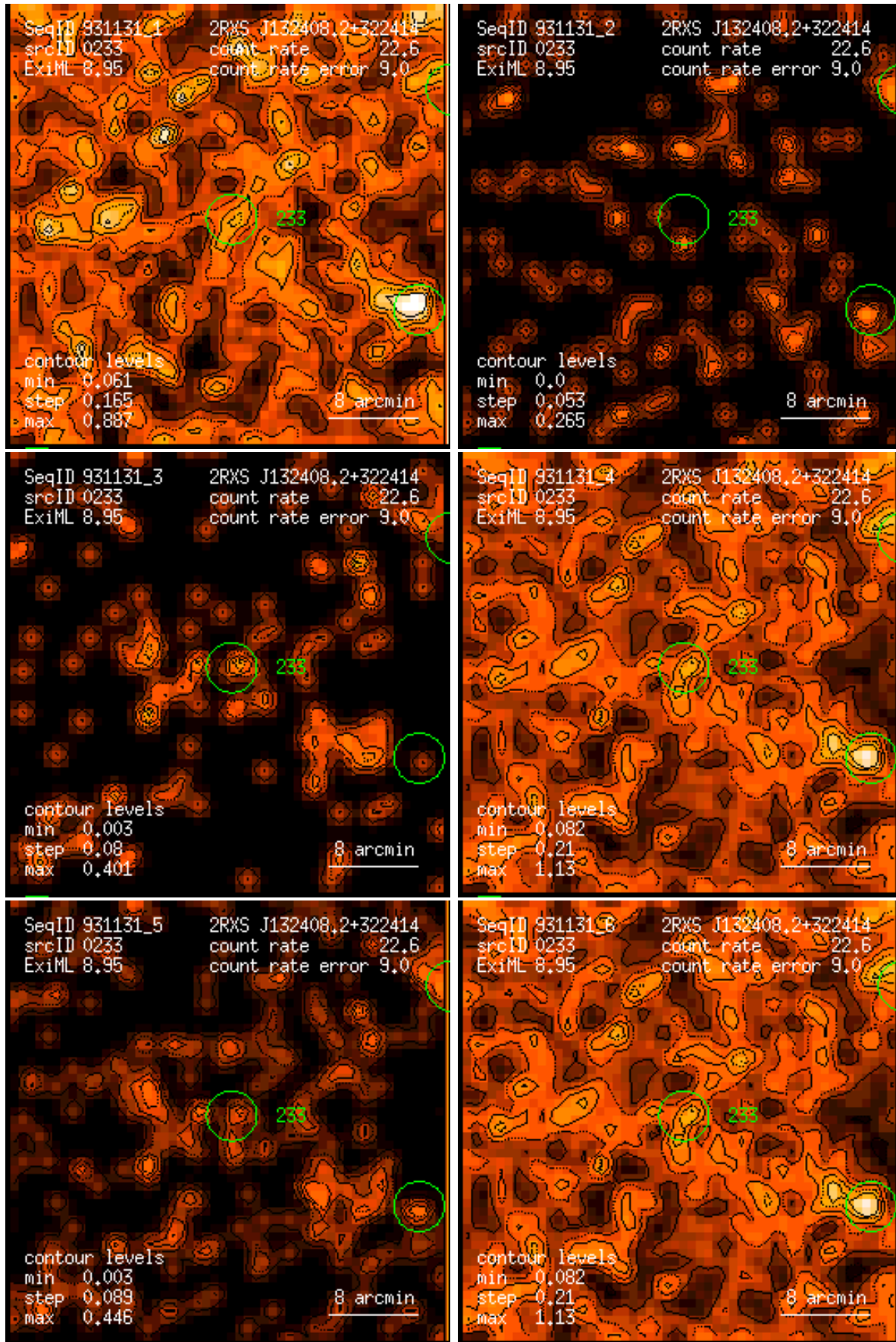
Figure 233: RASS 931131: detection 0233: band rate images, Gaussian filter: (1) PSPC channels 11 – 41, (2) 52 – 90, (3) 91 – 201, (4) 11 – 235, (5) 52 – 201, (6) 11 – 201. Broad band rates in counts/ks. Band rate contour levels in counts/ks/arcmin 2 .
