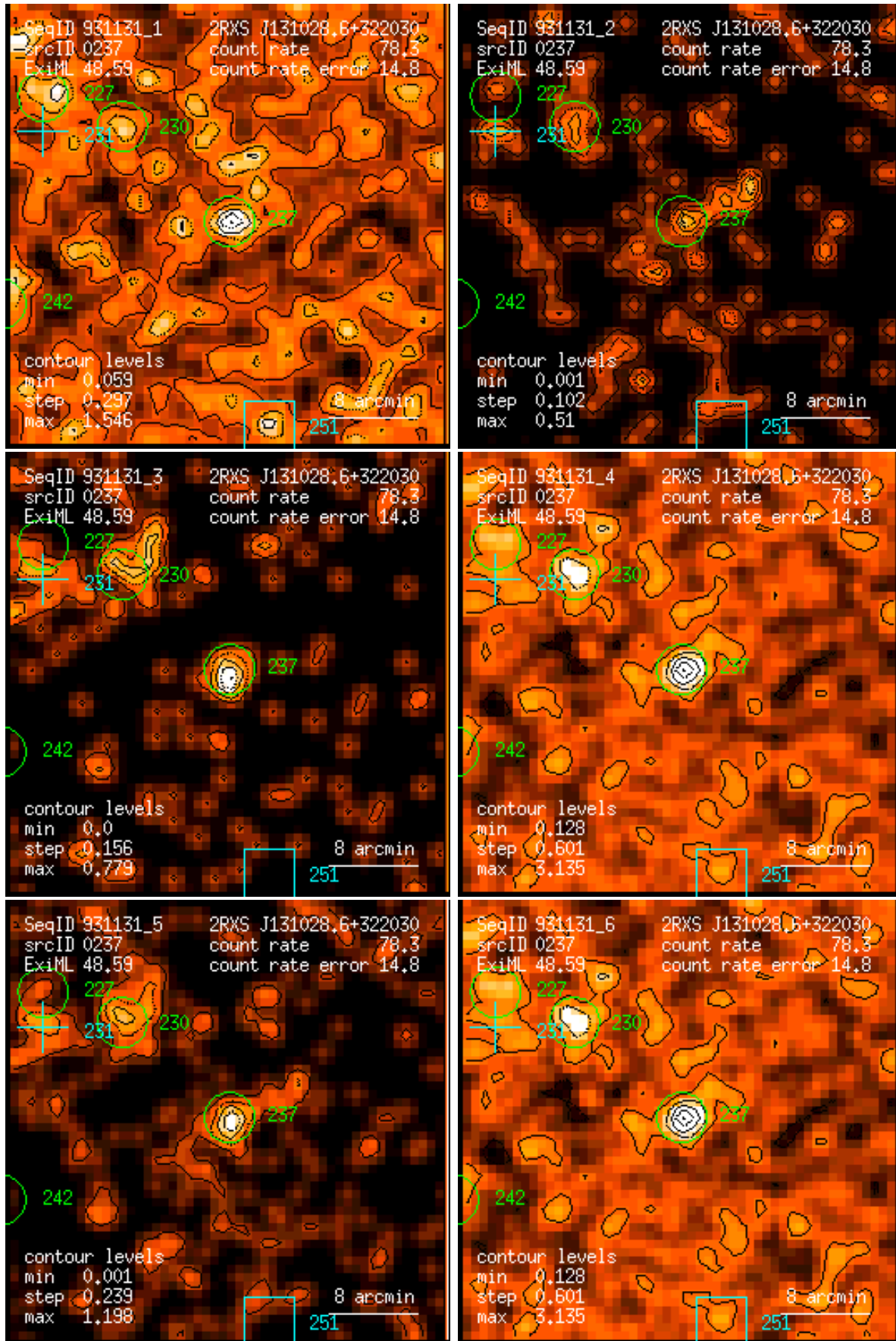
Figure 237: RASS 931131: detection 0237: band rate images, Gaussian filter: (1) PSPC channels 11 – 41, (2) 52 – 90, (3) 91 – 201, (4) 11 – 235, (5) 52 – 201, (6) 11 – 201. Broad band rates in counts/ks. Band rate contour levels in counts/ks/arcmin 2 .
