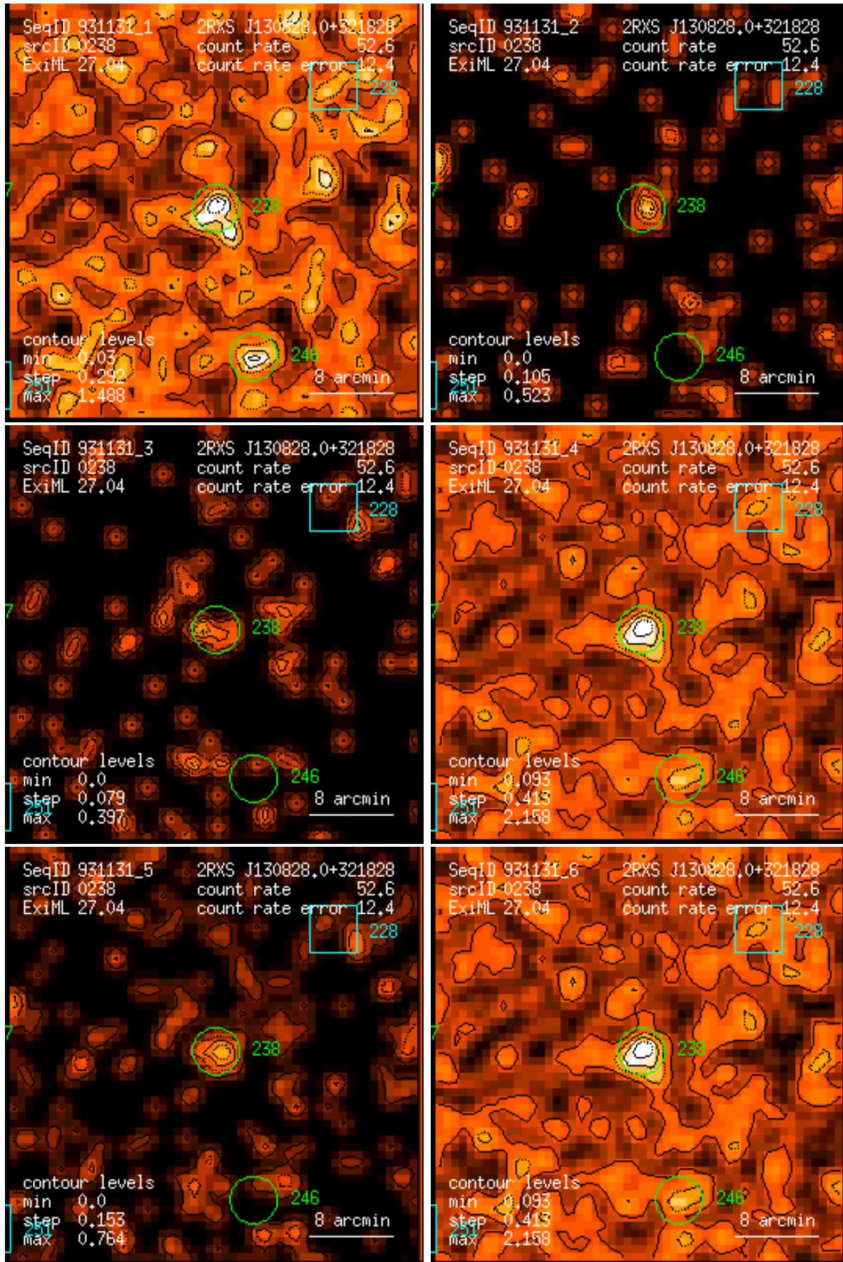
Figure 238: RASS 931131: detection 0238: band rate images, Gaussian filter: (1) PSPC channels 11 – 41, (2) 52 – 90, (3) 91 – 201, (4) 11 – 235, (5) 52 – 201, (6) 11 – 201. Broad band rates in counts/ks. Band rate contour levels in counts/ks/arcmin 2 .
