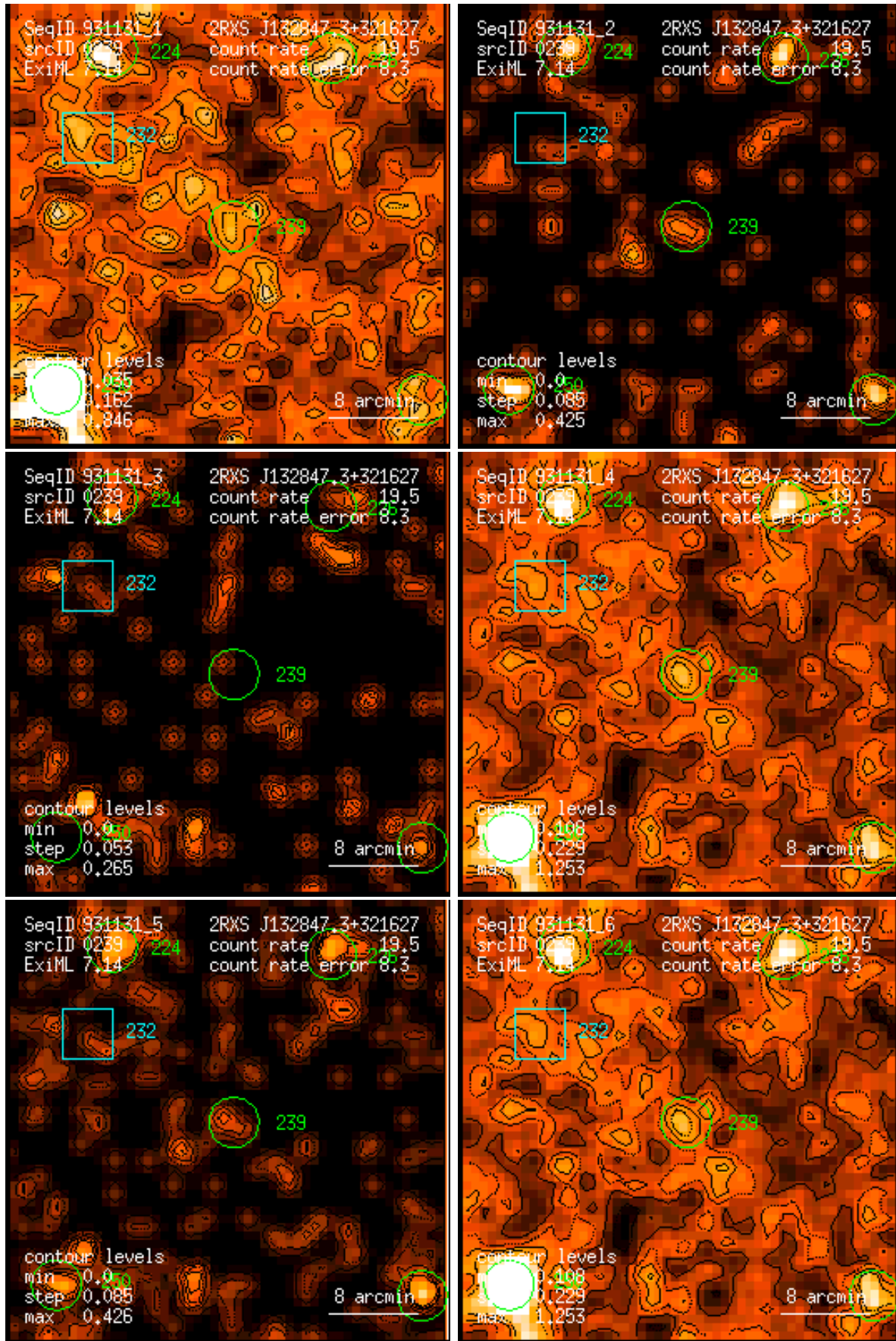
Figure 239: RASS 931131: detection 0239: band rate images, Gaussian filter: (1) PSPC channels 11 – 41, (2) 52 – 90, (3) 91 – 201, (4) 11 – 235, (5) 52 – 201, (6) 11 – 201. Broad band rates in counts/ks. Band rate contour levels in counts/ks/arcmin 2 .
