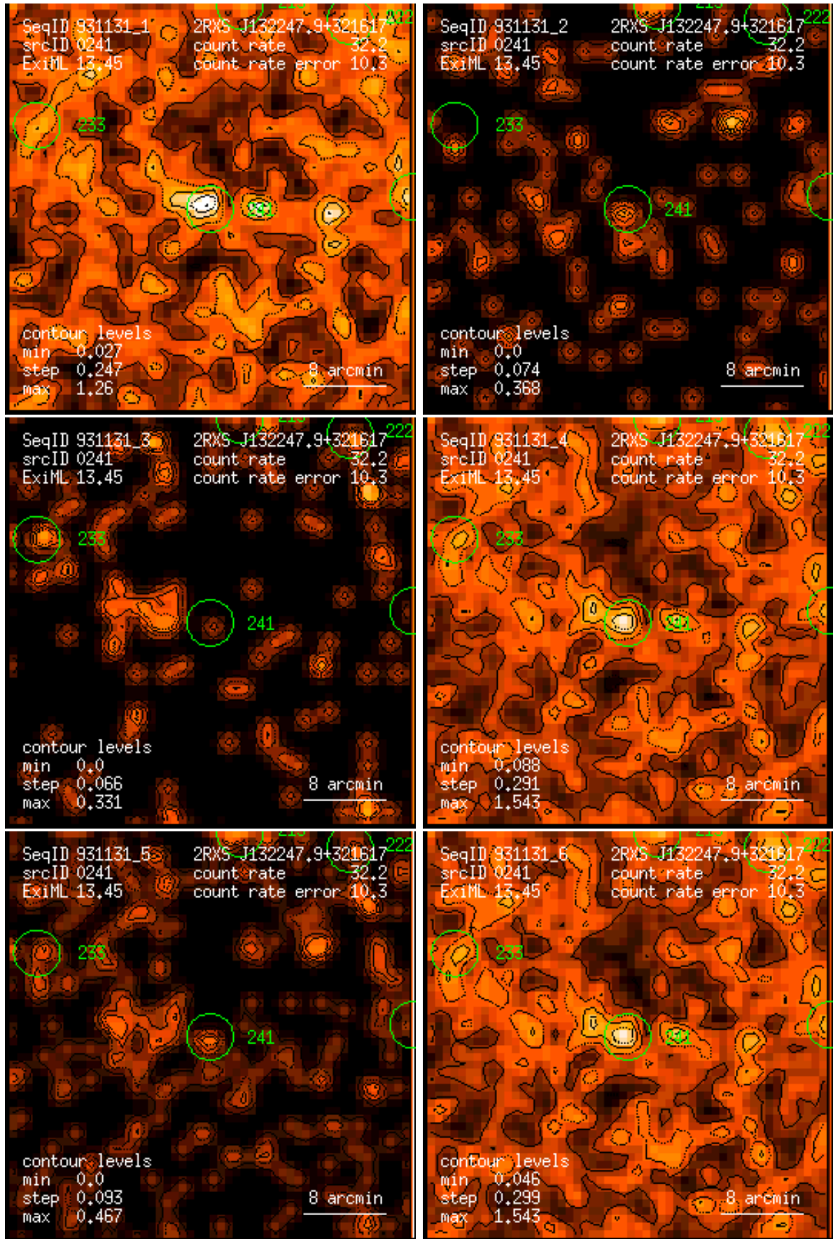
Figure 241: RASS 931131: detection 0241: band rate images, Gaussian filter: (1) PSPC channels 11 – 41, (2) 52 – 90, (3) 91 – 201, (4) 11 – 235, (5) 52 – 201, (6) 11 – 201. Broad band rates in counts/ks. Band rate contour levels in counts/ks/arcmin 2 .
