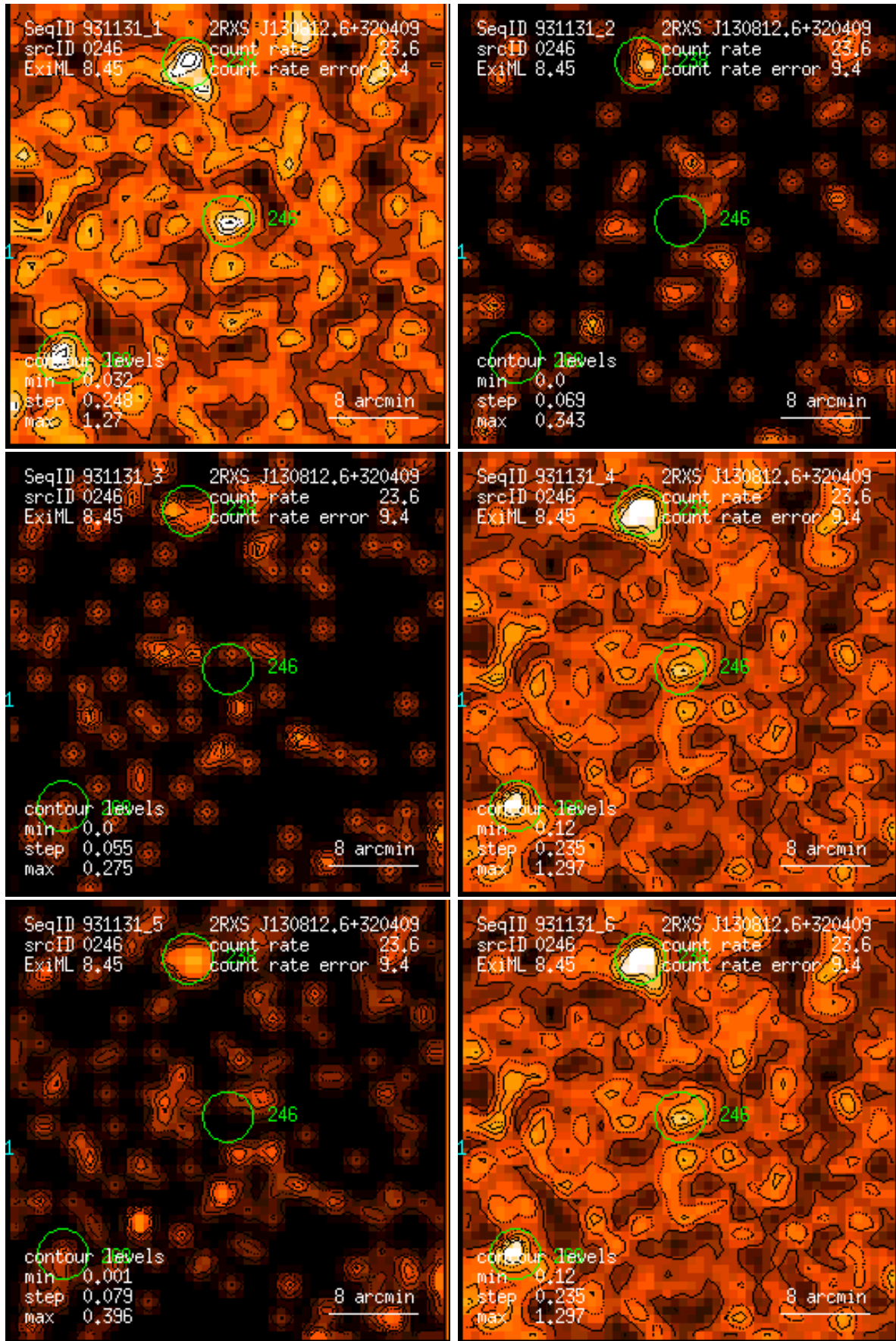
Figure 246: RASS 931131: detection 0246: band rate images, Gaussian filter: (1) PSPC channels 11 – 41, (2) 52 – 90, (3) 91 – 201, (4) 11 – 235, (5) 52 – 201, (6) 11 – 201. Broad band rates in counts/ks. Band rate contour levels in counts/ks/arcmin 2 .
