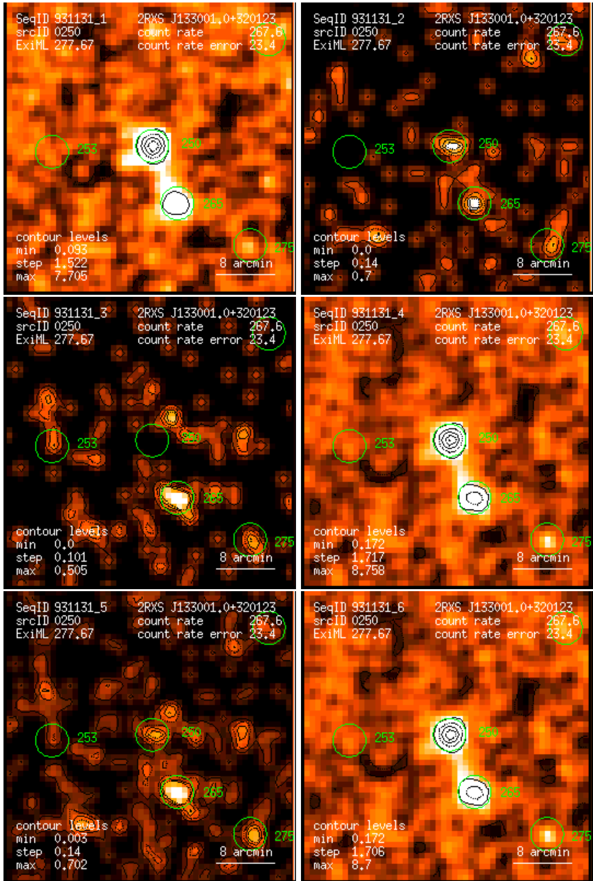
Figure 250: RASS 931131: detection 0250: band rate images, Gaussian filter: (1) PSPC channels 11 – 41, (2) 52 – 90, (3) 91 – 201, (4) 11 – 235, (5) 52 – 201, (6) 11 – 201. Broad band rates in counts/ks. Band rate contour levels in counts/ks/arcmin 2 .
