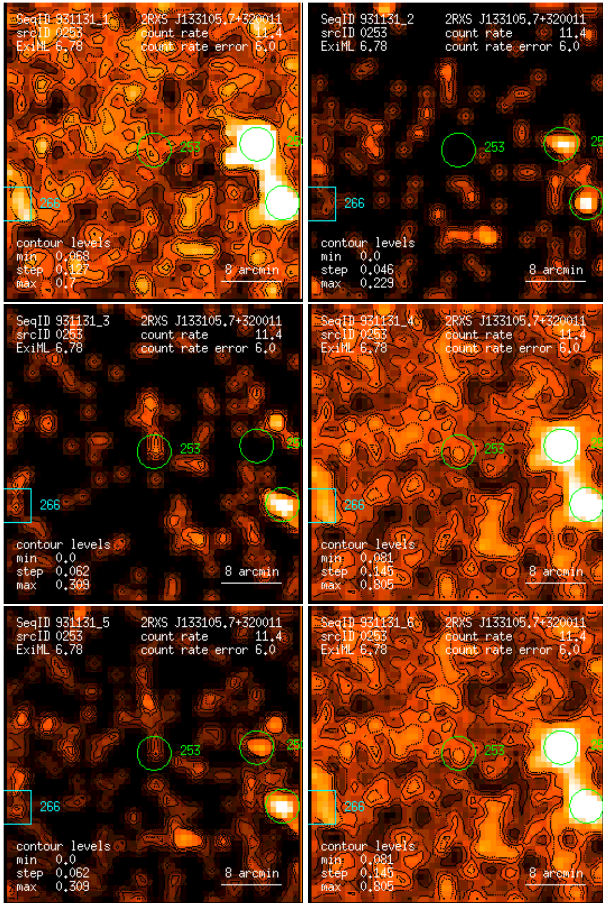
Figure 253: RASS 931131: detection 0253: band rate images, Gaussian filter: (1) PSPC channels 11 – 41, (2) 52 – 90, (3) 91 – 201, (4) 11 – 235, (5) 52 – 201, (6) 11 – 201. Broad band rates in counts/ks. Band rate contour levels in counts/ks/arcmin 2 .
