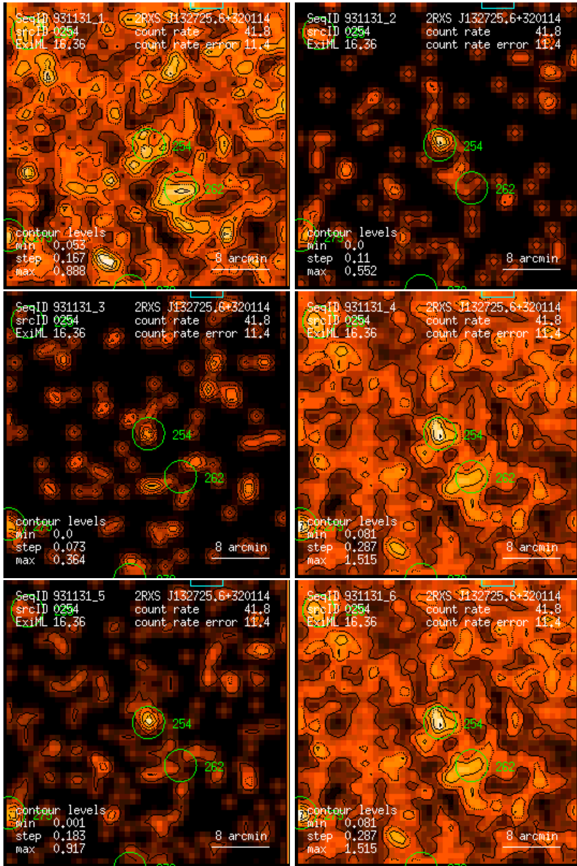
Figure 254: RASS 931131: detection 0254: band rate images, Gaussian filter: (1) PSPC channels 11 – 41, (2) 52 – 90, (3) 91 – 201, (4) 11 – 235, (5) 52 – 201, (6) 11 – 201. Broad band rates in counts/ks. Band rate contour levels in counts/ks/arcmin 2 .
