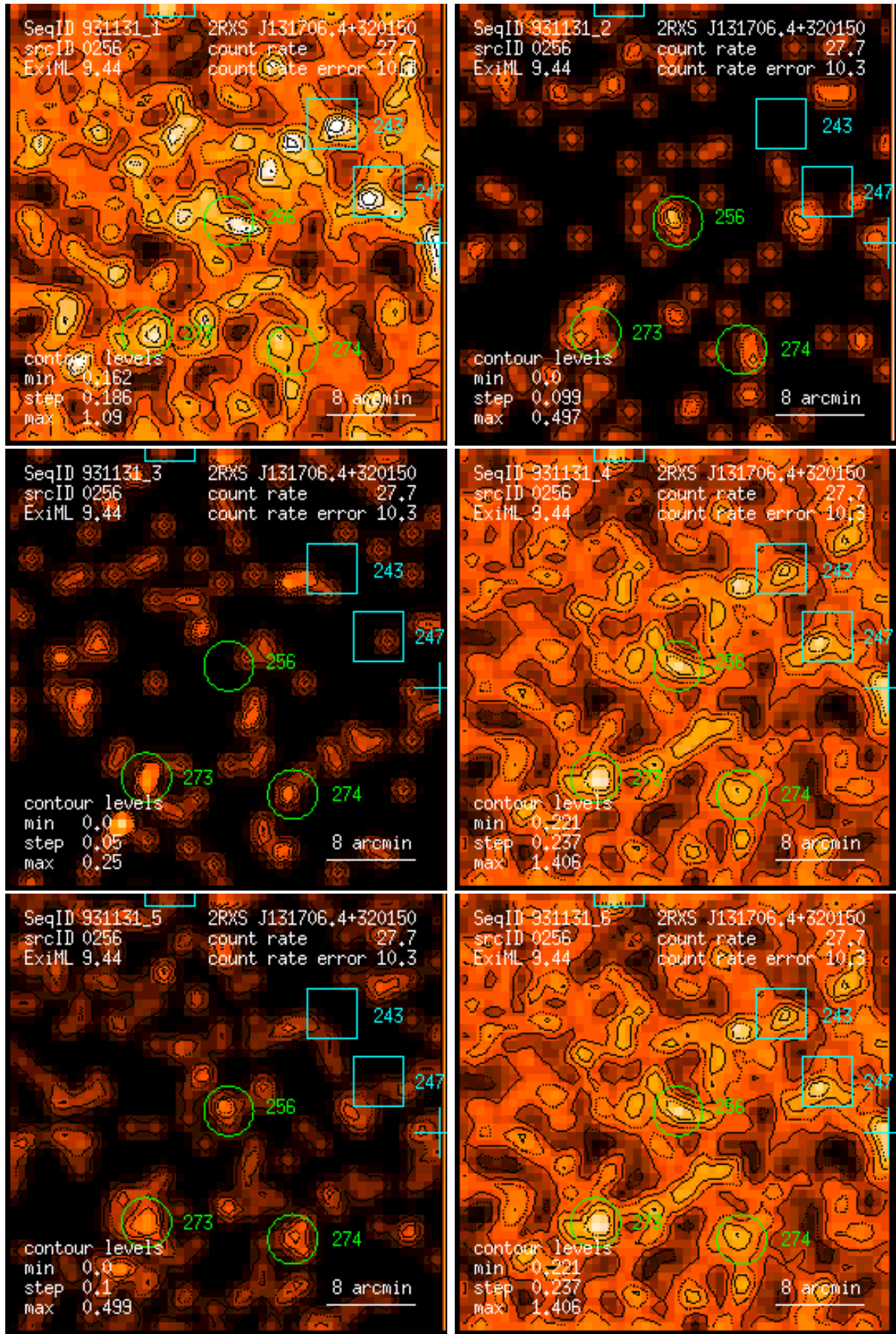
Figure 256: RASS 931131: detection 0256: band rate images, Gaussian filter: (1) PSPC channels 11 – 41, (2) 52 – 90, (3) 91 – 201, (4) 11 – 235, (5) 52 – 201, (6) 11 – 201. Broad band rates in counts/ks. Band rate contour levels in counts/ks/arcmin 2 .
