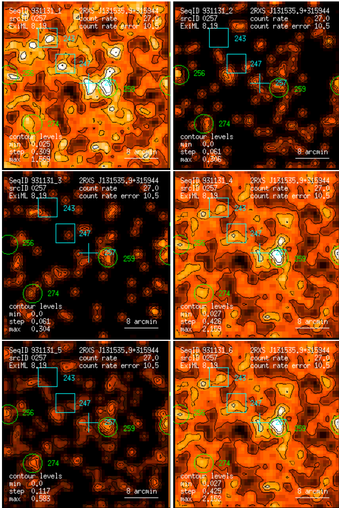
Figure 257: RASS 931131: detection 0257: band rate images, Gaussian filter: (1) PSPC channels 11 – 41, (2) 52 – 90, (3) 91 – 201, (4) 11 – 235, (5) 52 – 201, (6) 11 – 201. Broad band rates in counts/ks. Band rate contour levels in counts/ks/arcmin 2 .
