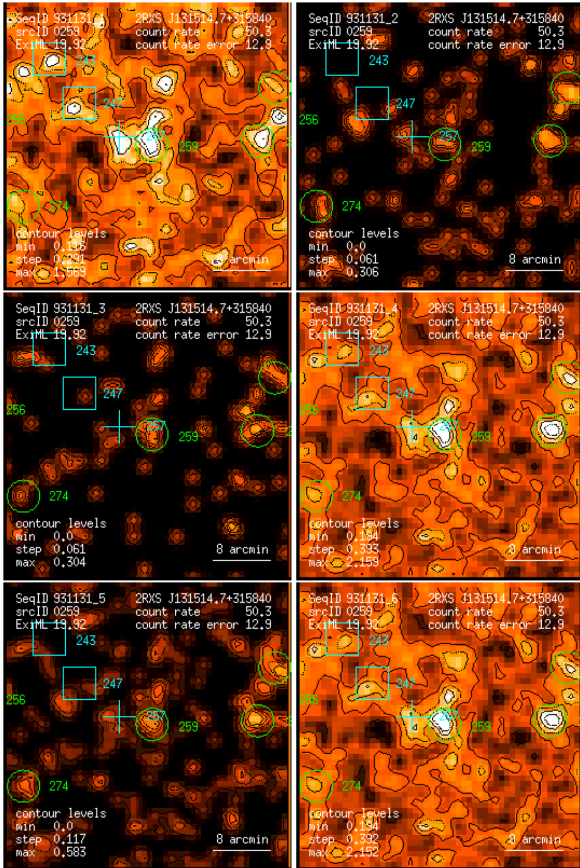
Figure 259: RASS 931131: detection 0259: band rate images, Gaussian filter: (1) PSPC channels 11 – 41, (2) 52 – 90, (3) 91 – 201, (4) 11 – 235, (5) 52 – 201, (6) 11 – 201. Broad band rates in counts/ks. Band rate contour levels in counts/ks/arcmin 2 .
