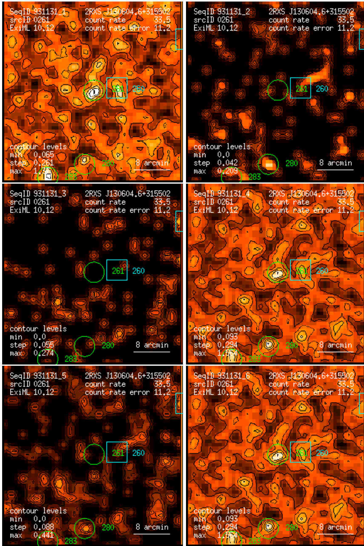
Figure 261: RASS 931131: detection 0261: band rate images, Gaussian filter: (1) PSPC channels 11 – 41, (2) 52 – 90, (3) 91 – 201, (4) 11 – 235, (5) 52 – 201, (6) 11 – 201. Broad band rates in counts/ks. Band rate contour levels in counts/ks/arcmin 2 .
