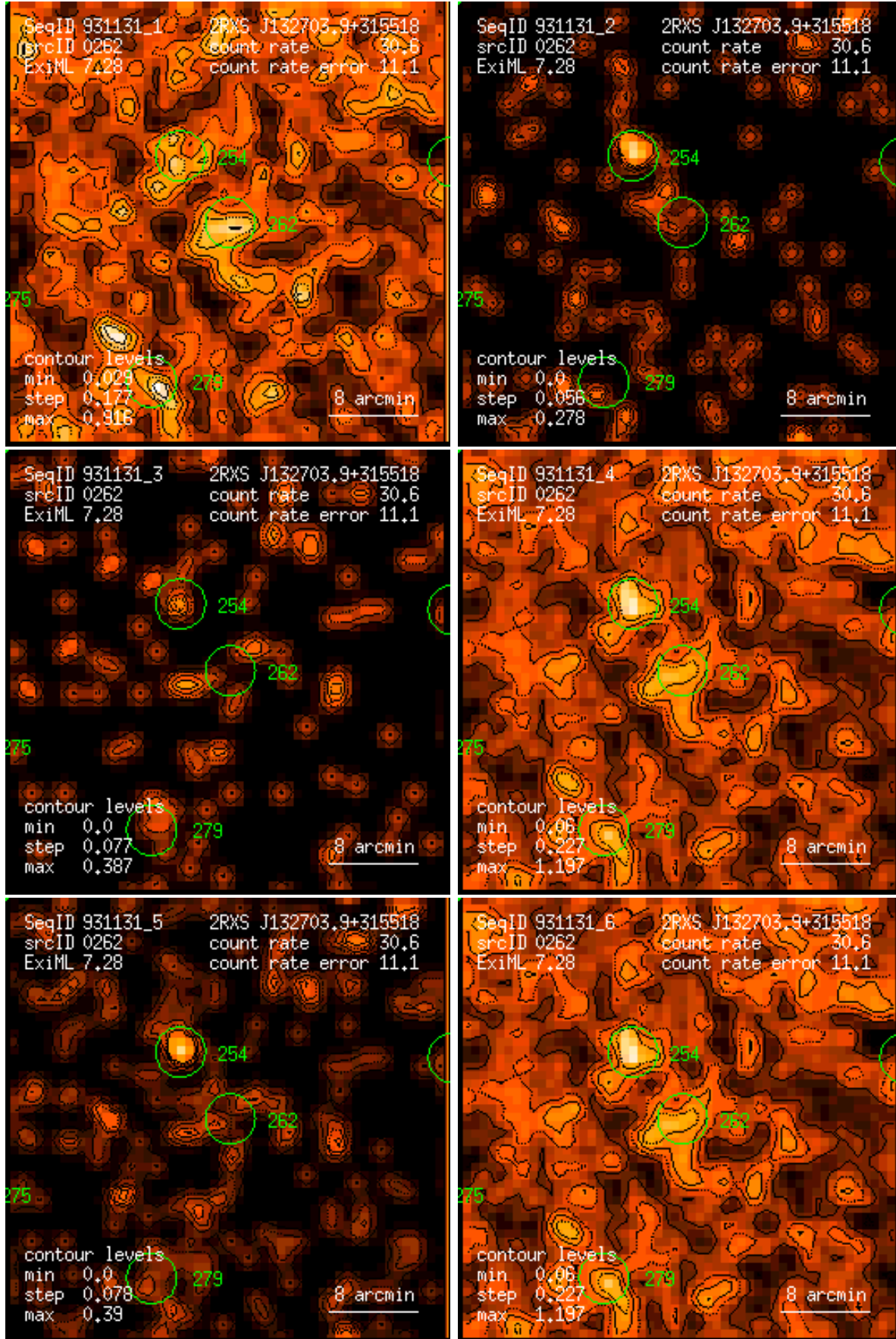
Figure 262: RASS 931131: detection 0262: band rate images, Gaussian filter: (1) PSPC channels 11 – 41, (2) 52 – 90, (3) 91 – 201, (4) 11 – 235, (5) 52 – 201, (6) 11 – 201. Broad band rates in counts/ks. Band rate contour levels in counts/ks/arcmin 2 .
