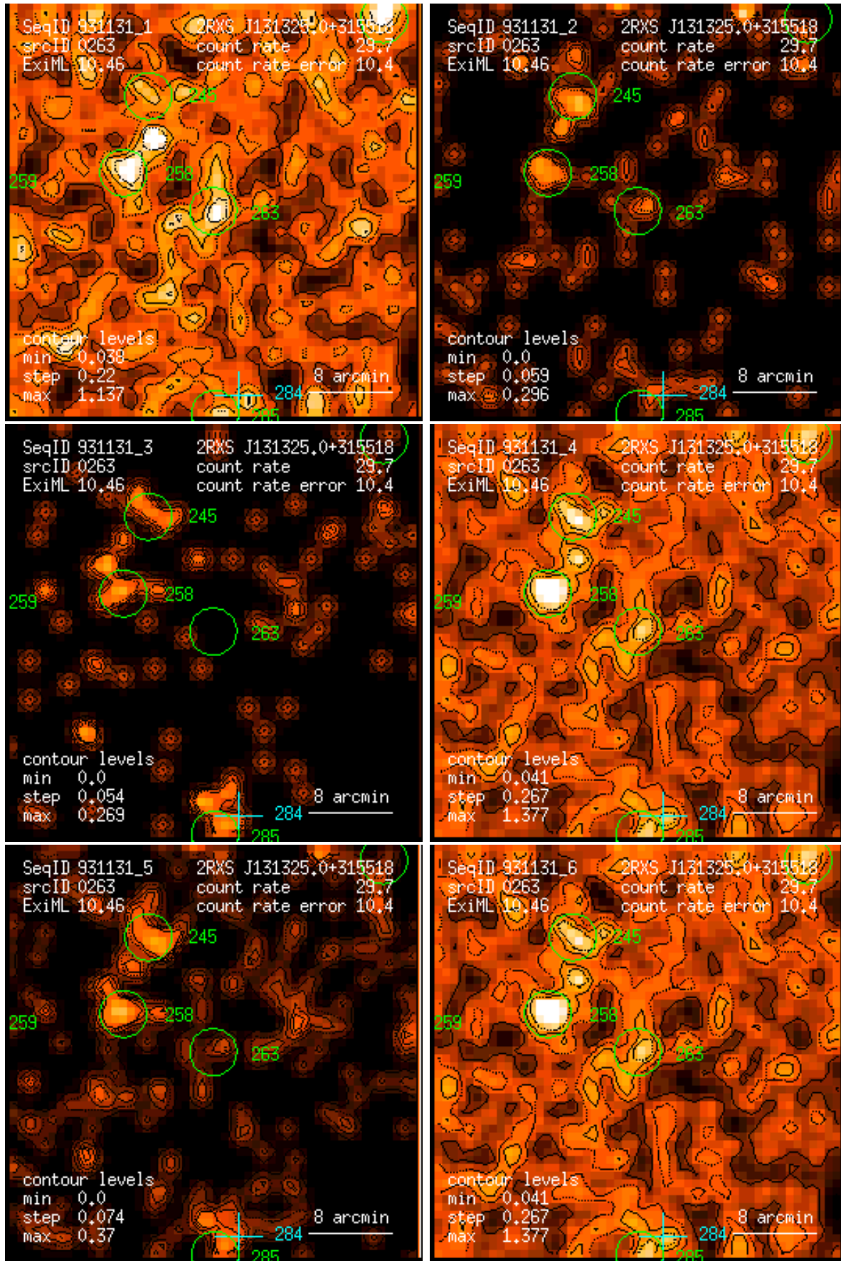
Figure 263: RASS 931131: detection 0263: band rate images, Gaussian filter: (1) PSPC channels 11 – 41, (2) 52 – 90, (3) 91 – 201, (4) 11 – 235, (5) 52 – 201, (6) 11 – 201. Broad band rates in counts/ks. Band rate contour levels in counts/ks/arcmin 2 .
