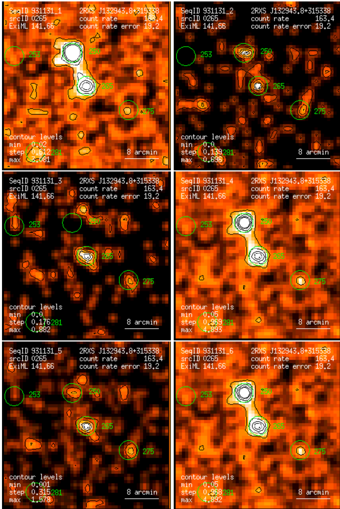
Figure 265: RASS 931131: detection 0265: band rate images, Gaussian filter: (1) PSPC channels 11 – 41, (2) 52 – 90, (3) 91 – 201, (4) 11 – 235, (5) 52 – 201, (6) 11 – 201. Broad band rates in counts/ks. Band rate contour levels in counts/ks/arcmin 2 .
