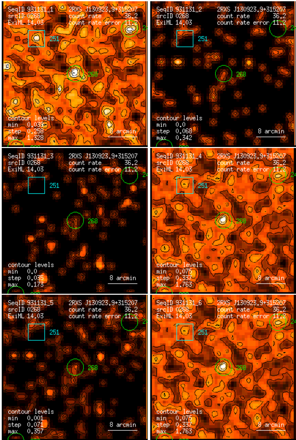
Figure 268: RASS 931131: detection 0268: band rate images, Gaussian filter: (1) PSPC channels 11 – 41, (2) 52 – 90, (3) 91 – 201, (4) 11 – 235, (5) 52 – 201, (6) 11 – 201. Broad band rates in counts/ks. Band rate contour levels in counts/ks/arcmin 2 .
