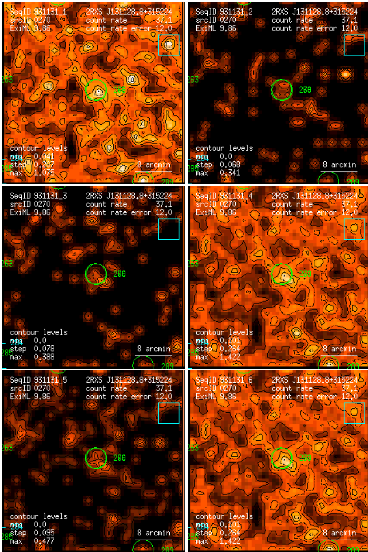
Figure 270: RASS 931131: detection 0270: band rate images, Gaussian filter: (1) PSPC channels 11 – 41, (2) 52 – 90, (3) 91 – 201, (4) 11 – 235, (5) 52 – 201, (6) 11 – 201. Broad band rates in counts/ks. Band rate contour levels in counts/ks/arcmin 2 .
