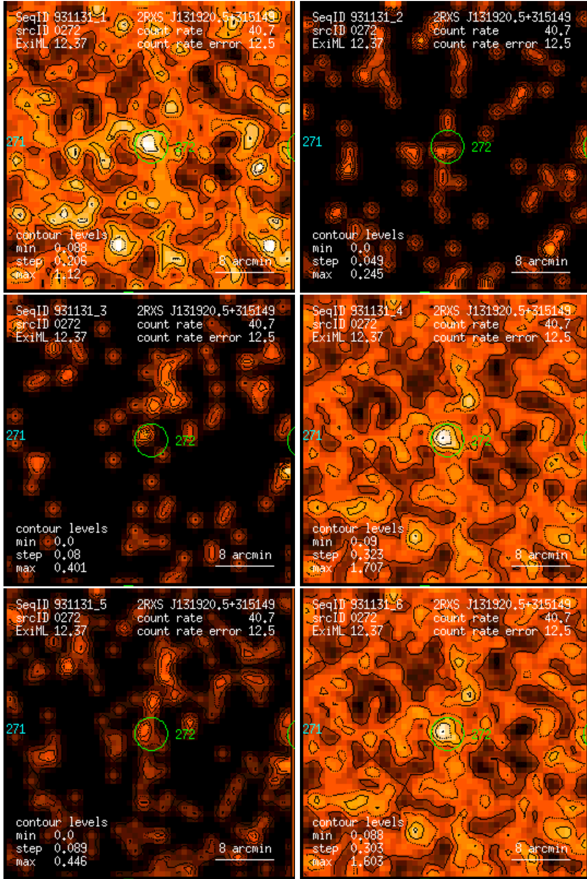
Figure 272: RASS 931131: detection 0272: band rate images, Gaussian filter: (1) PSPC channels 11 – 41, (2) 52 – 90, (3) 91 – 201, (4) 11 – 235, (5) 52 – 201, (6) 11 – 201. Broad band rates in counts/ks. Band rate contour levels in counts/ks/arcmin 2 .
