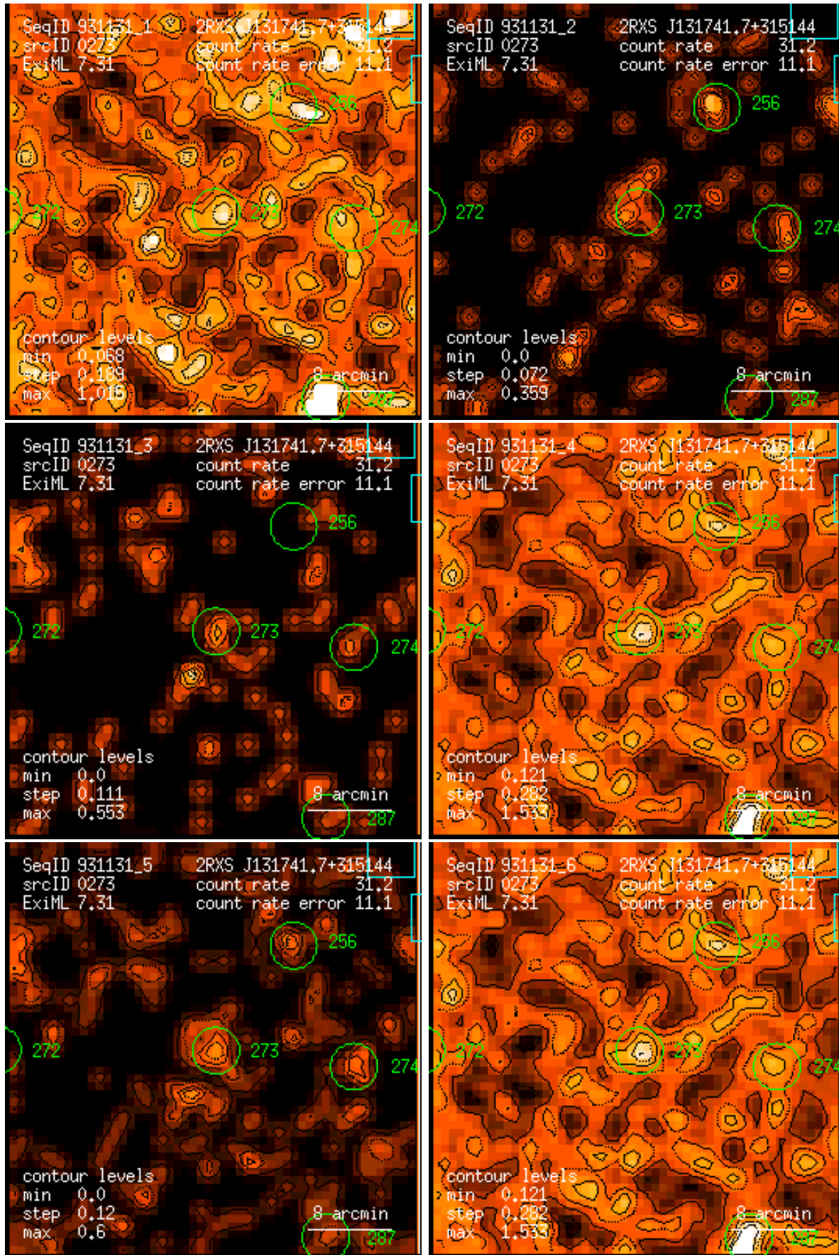
Figure 273: RASS 931131: detection 0273: band rate images, Gaussian filter: (1) PSPC channels 11 – 41, (2) 52 – 90, (3) 91 – 201, (4) 11 – 235, (5) 52 – 201, (6) 11 – 201. Broad band rates in counts/ks. Band rate contour levels in counts/ks/arcmin 2 .
