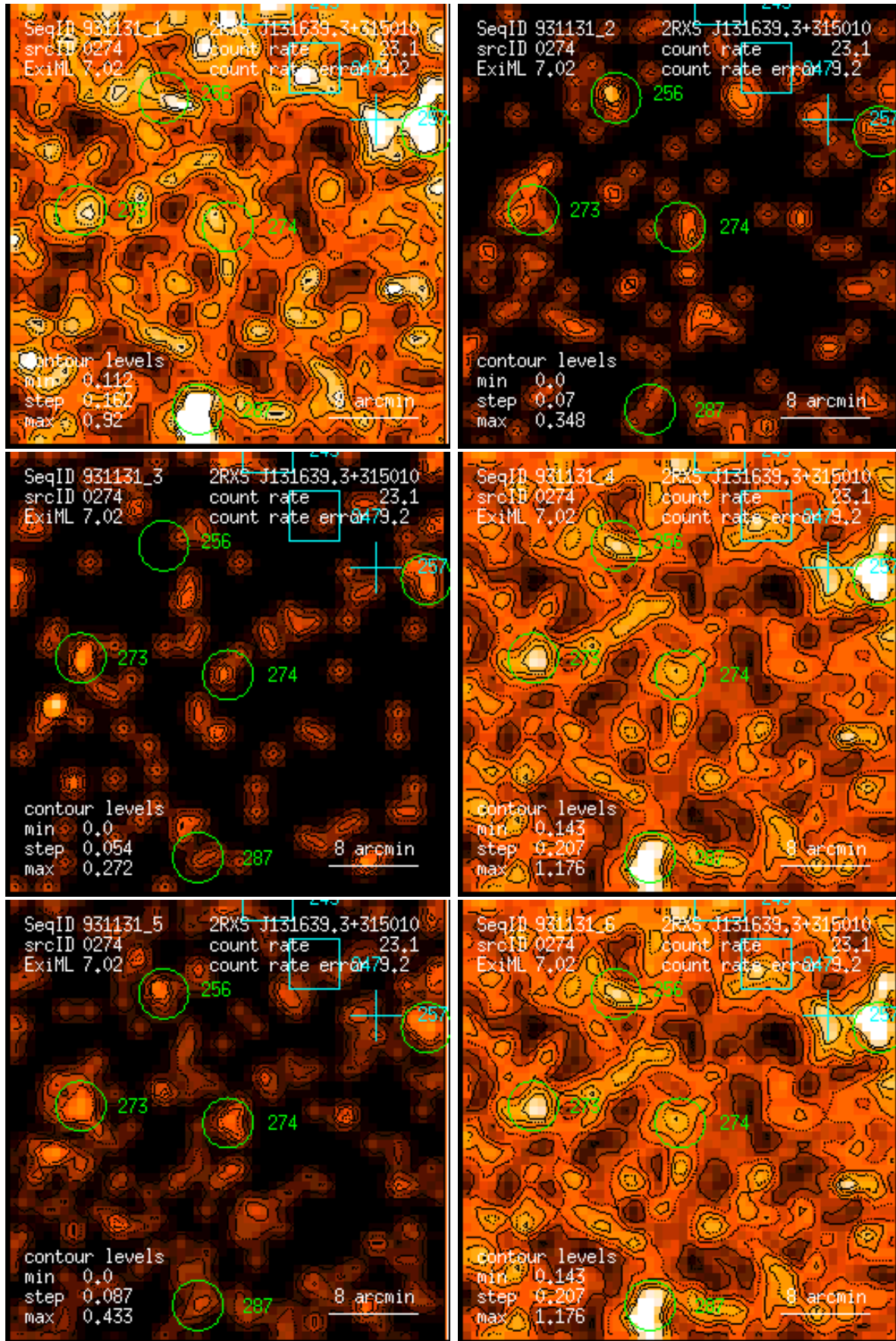
Figure 274: RASS 931131: detection 0274: band rate images, Gaussian filter: (1) PSPC channels 11 – 41, (2) 52 – 90, (3) 91 – 201, (4) 11 – 235, (5) 52 – 201, (6) 11 – 201. Broad band rates in counts/ks. Band rate contour levels in counts/ks/arcmin 2 .
