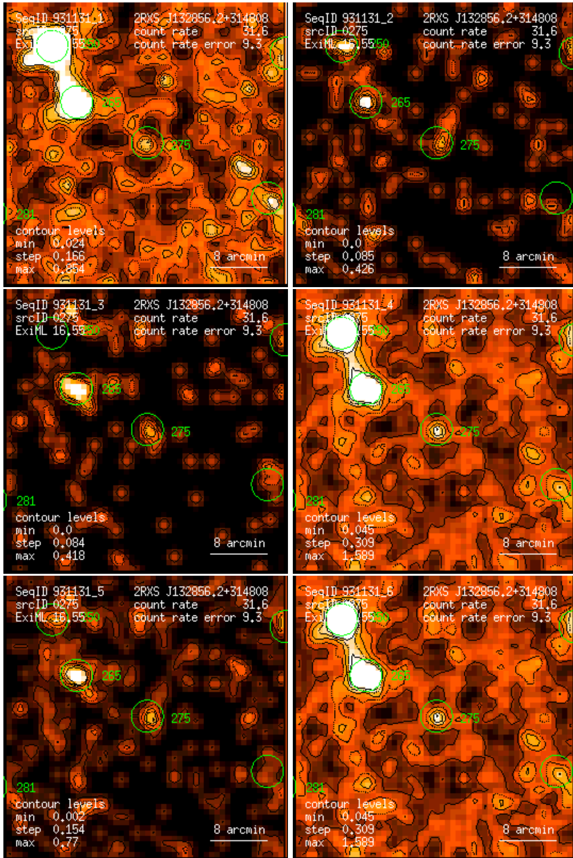
Figure 275: RASS 931131: detection 0275: band rate images, Gaussian filter: (1) PSPC channels 11 – 41, (2) 52 – 90, (3) 91 – 201, (4) 11 – 235, (5) 52 – 201, (6) 11 – 201. Broad band rates in counts/ks. Band rate contour levels in counts/ks/arcmin 2 .
