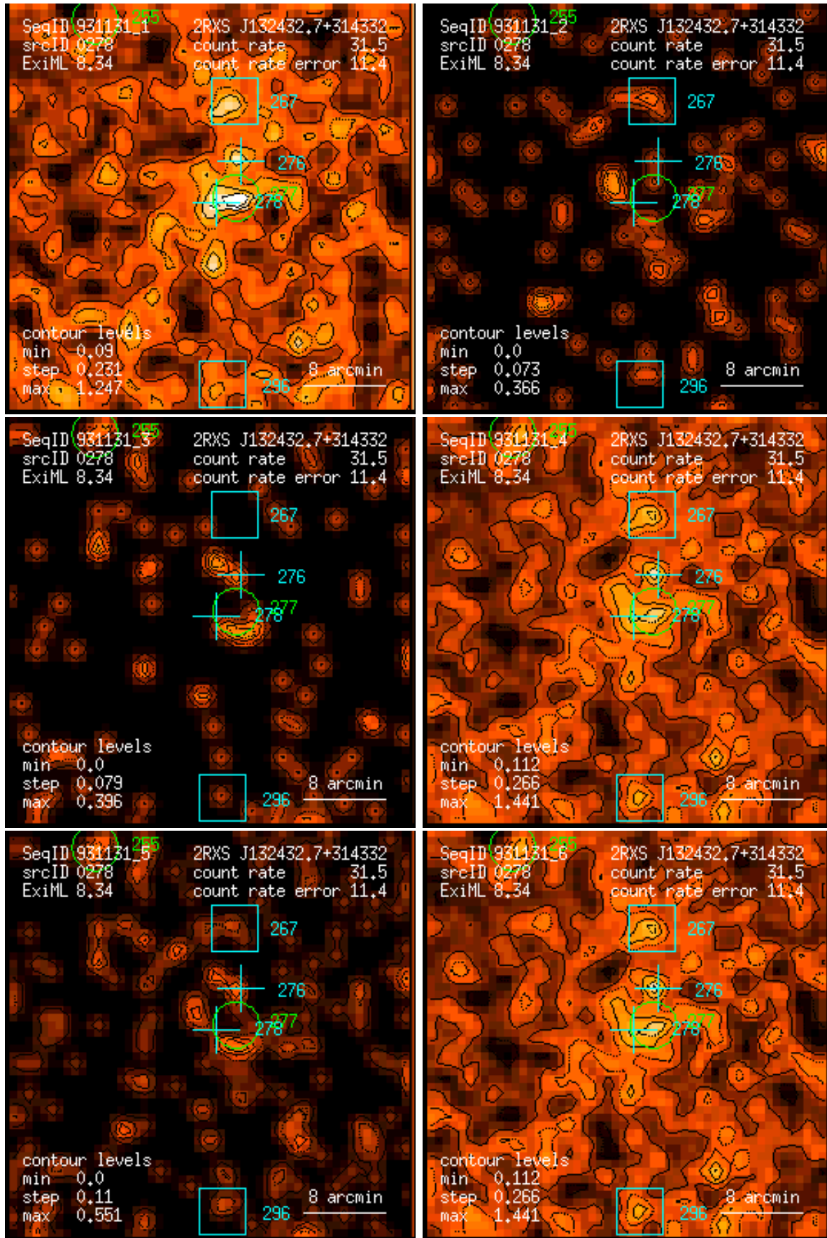
Figure 278: RASS 931131: detection 0278: band rate images, Gaussian filter: (1) PSPC channels 11 – 41, (2) 52 – 90, (3) 91 – 201, (4) 11 – 235, (5) 52 – 201, (6) 11 – 201. Broad band rates in counts/ks. Band rate contour levels in counts/ks/arcmin 2 .
