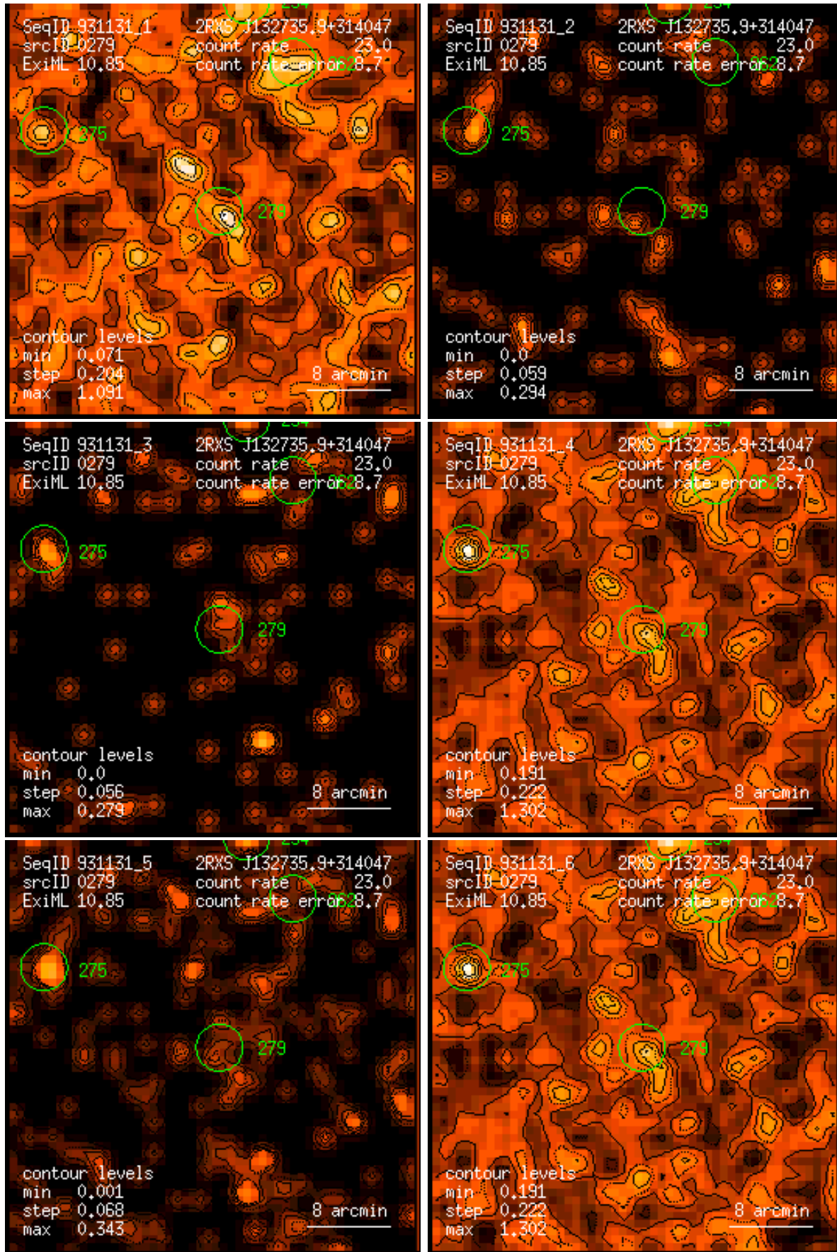
Figure 279: RASS 931131: detection 0279: band rate images, Gaussian filter: (1) PSPC channels 11 – 41, (2) 52 – 90, (3) 91 – 201, (4) 11 – 235, (5) 52 – 201, (6) 11 – 201. Broad band rates in counts/ks. Band rate contour levels in counts/ks/arcmin 2 .
