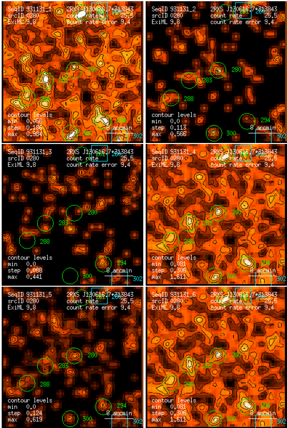
Figure 280: RASS 931131: detection 0280: band rate images, Gaussian filter: (1) PSPC channels 11 – 41, (2) 52 – 90, (3) 91 – 201, (4) 11 – 235, (5) 52 – 201, (6) 11 – 201. Broad band rates in counts/ks. Band rate contour levels in counts/ks/arcmin 2 .
