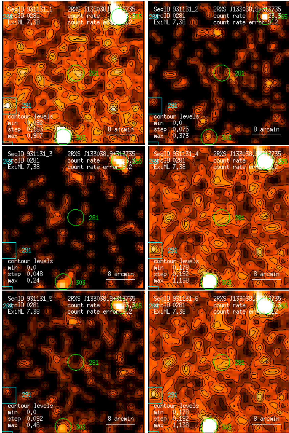
Figure 281: RASS 931131: detection 0281: band rate images, Gaussian filter: (1) PSPC channels 11 – 41, (2) 52 – 90, (3) 91 – 201, (4) 11 – 235, (5) 52 – 201, (6) 11 – 201. Broad band rates in counts/ks. Band rate contour levels in counts/ks/arcmin 2 .
