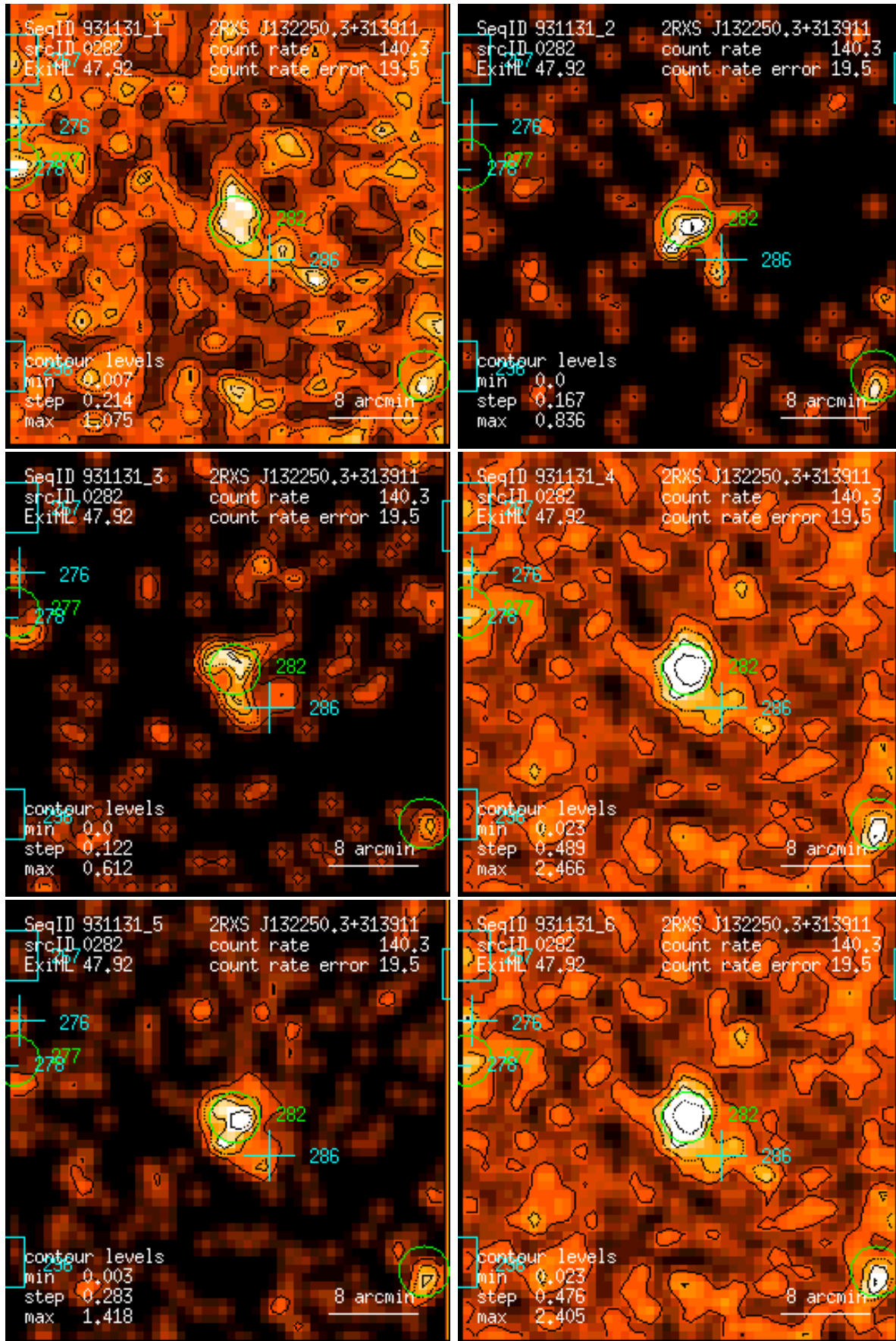
Figure 282: RASS 931131: detection 0282: band rate images, Gaussian filter: (1) PSPC channels 11 – 41, (2) 52 – 90, (3) 91 – 201, (4) 11 – 235, (5) 52 – 201, (6) 11 – 201. Broad band rates in counts/ks. Band rate contour levels in counts/ks/arcmin 2 .
