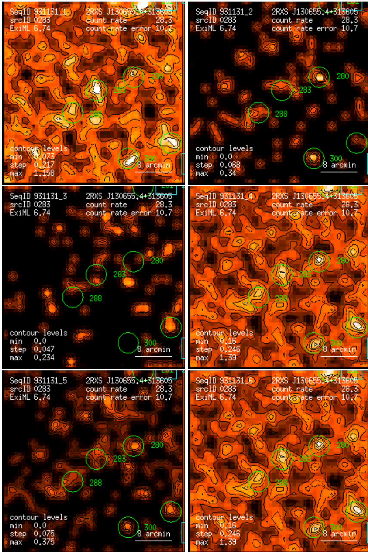
Figure 283: RASS 931131: detection 0283: band rate images, Gaussian filter: (1) PSPC channels 11 – 41, (2) 52 – 90, (3) 91 – 201, (4) 11 – 235, (5) 52 – 201, (6) 11 – 201. Broad band rates in counts/ks. Band rate contour levels in counts/ks/arcmin 2 .
