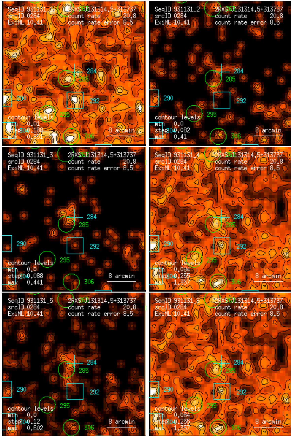
Figure 284: RASS 931131: detection 0284: band rate images, Gaussian filter: (1) PSPC channels 11 – 41, (2) 52 – 90, (3) 91 – 201, (4) 11 – 235, (5) 52 – 201, (6) 11 – 201. Broad band rates in counts/ks. Band rate contour levels in counts/ks/arcmin 2 .
