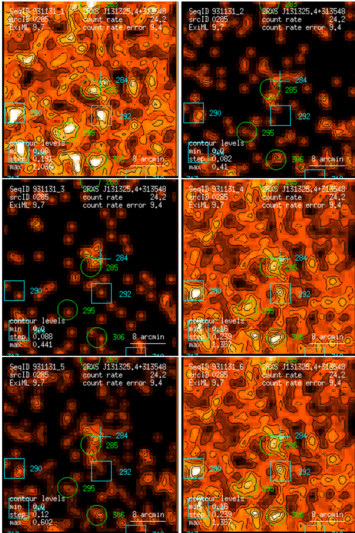
Figure 285: RASS 931131: detection 0285: band rate images, Gaussian filter: (1) PSPC channels 11 – 41, (2) 52 – 90, (3) 91 – 201, (4) 11 – 235, (5) 52 – 201, (6) 11 – 201. Broad band rates in counts/ks. Band rate contour levels in counts/ks/arcmin 2 .
