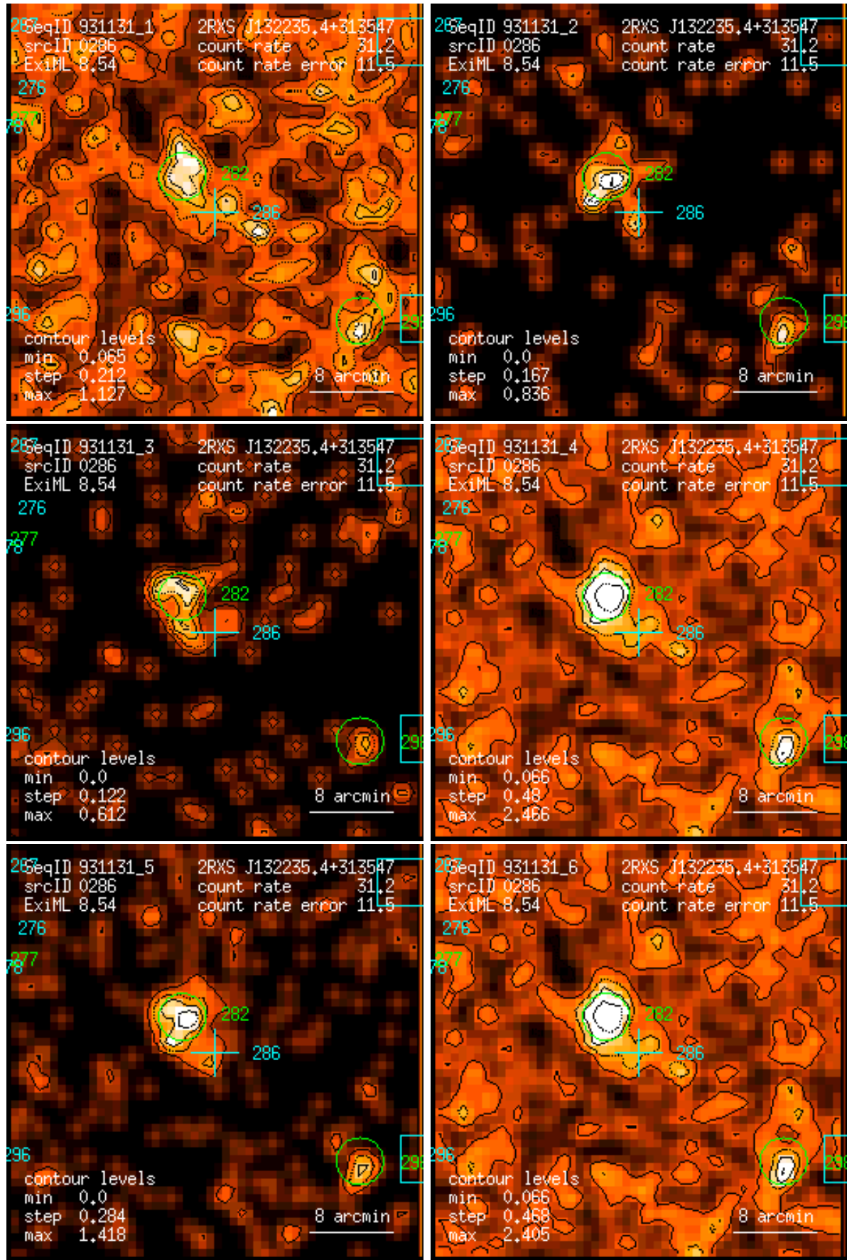
Figure 286: RASS 931131: detection 0286: band rate images, Gaussian filter: (1) PSPC channels 11 – 41, (2) 52 – 90, (3) 91 – 201, (4) 11 – 235, (5) 52 – 201, (6) 11 – 201. Broad band rates in counts/ks. Band rate contour levels in counts/ks/arcmin 2 .
