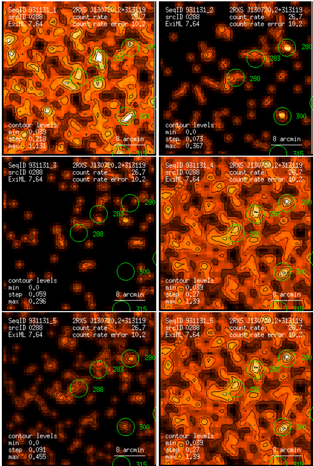
Figure 288: RASS 931131: detection 0288: band rate images, Gaussian filter: (1) PSPC channels 11 – 41, (2) 52 – 90, (3) 91 – 201, (4) 11 – 235, (5) 52 – 201, (6) 11 – 201. Broad band rates in counts/ks. Band rate contour levels in counts/ks/arcmin 2 .
