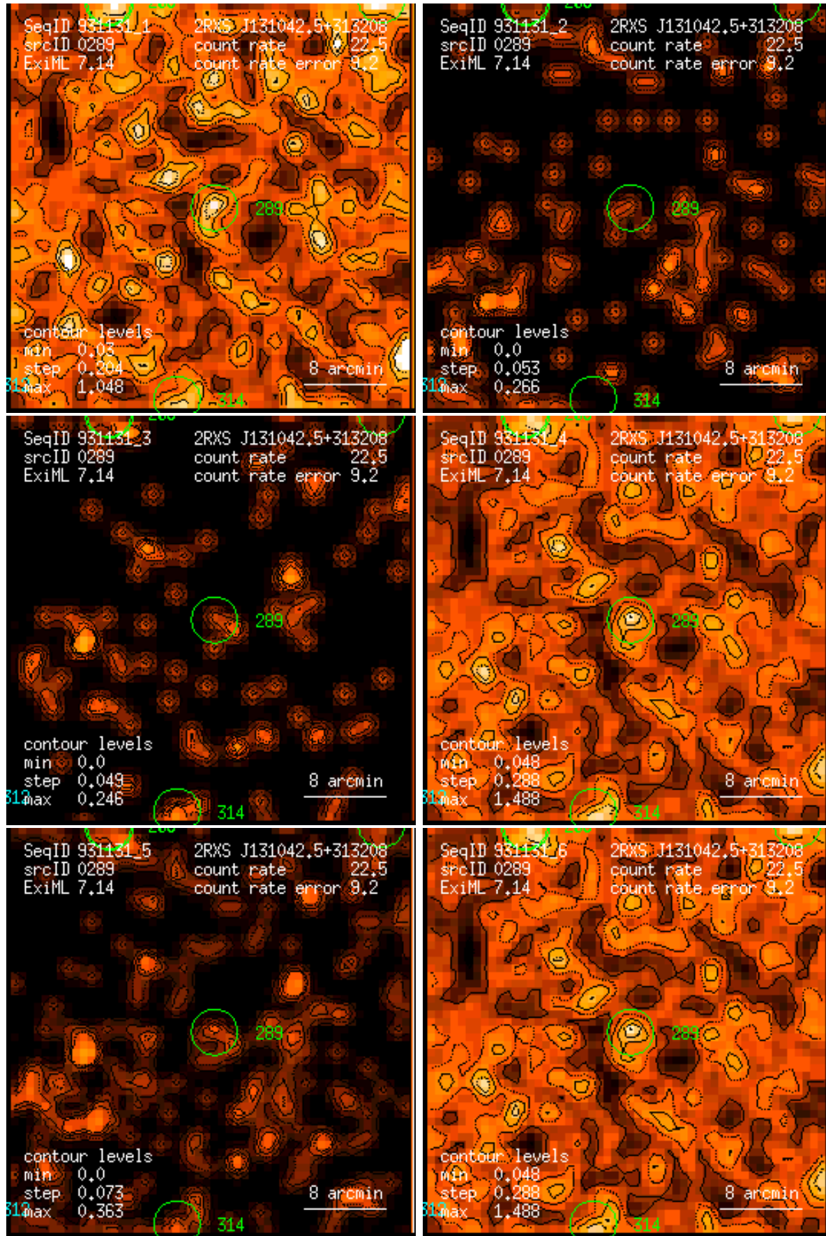
Figure 289: RASS 931131: detection 0289: band rate images, Gaussian filter: (1) PSPC channels 11 – 41, (2) 52 – 90, (3) 91 – 201, (4) 11 – 235, (5) 52 – 201, (6) 11 – 201. Broad band rates in counts/ks. Band rate contour levels in counts/ks/arcmin 2 .
