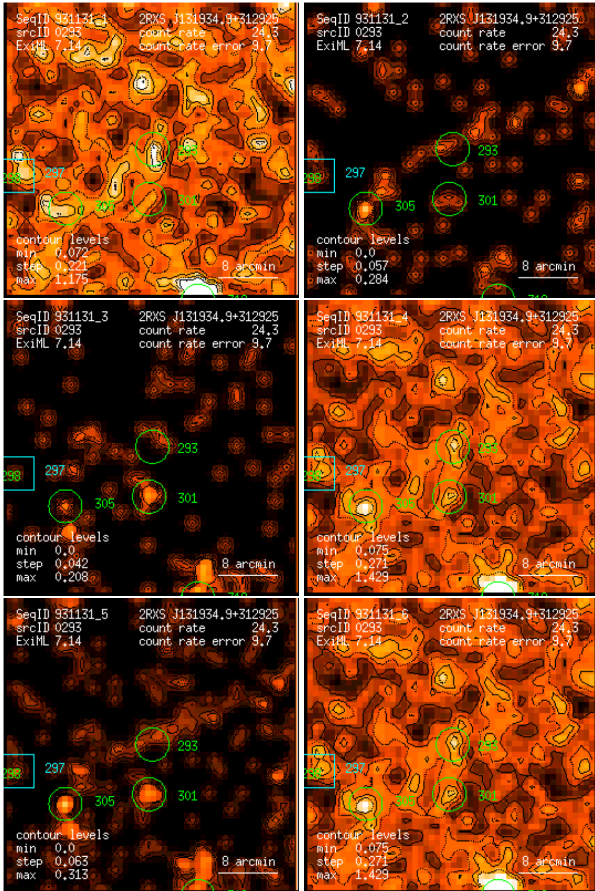
Figure 293: RASS 931131: detection 0293: band rate images, Gaussian filter: (1) PSPC channels 11 – 41, (2) 52 – 90, (3) 91 – 201, (4) 11 – 235, (5) 52 – 201, (6) 11 – 201. Broad band rates in counts/ks. Band rate contour levels in counts/ks/arcmin 2 .
