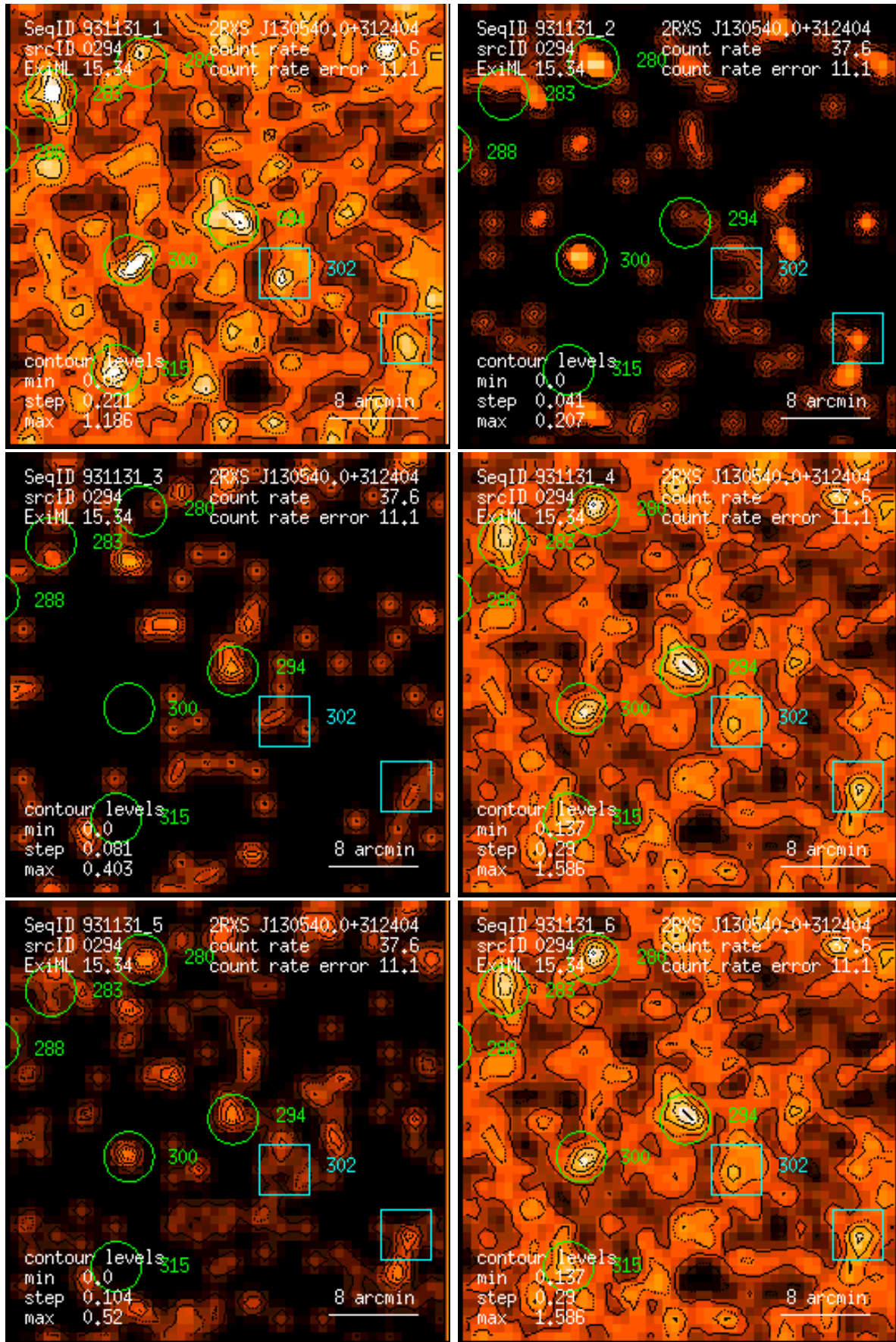
Figure 294: RASS 931131: detection 0294: band rate images, Gaussian filter: (1) PSPC channels 11 – 41, (2) 52 – 90, (3) 91 – 201, (4) 11 – 235, (5) 52 – 201, (6) 11 – 201. Broad band rates in counts/ks. Band rate contour levels in counts/ks/arcmin 2 .
