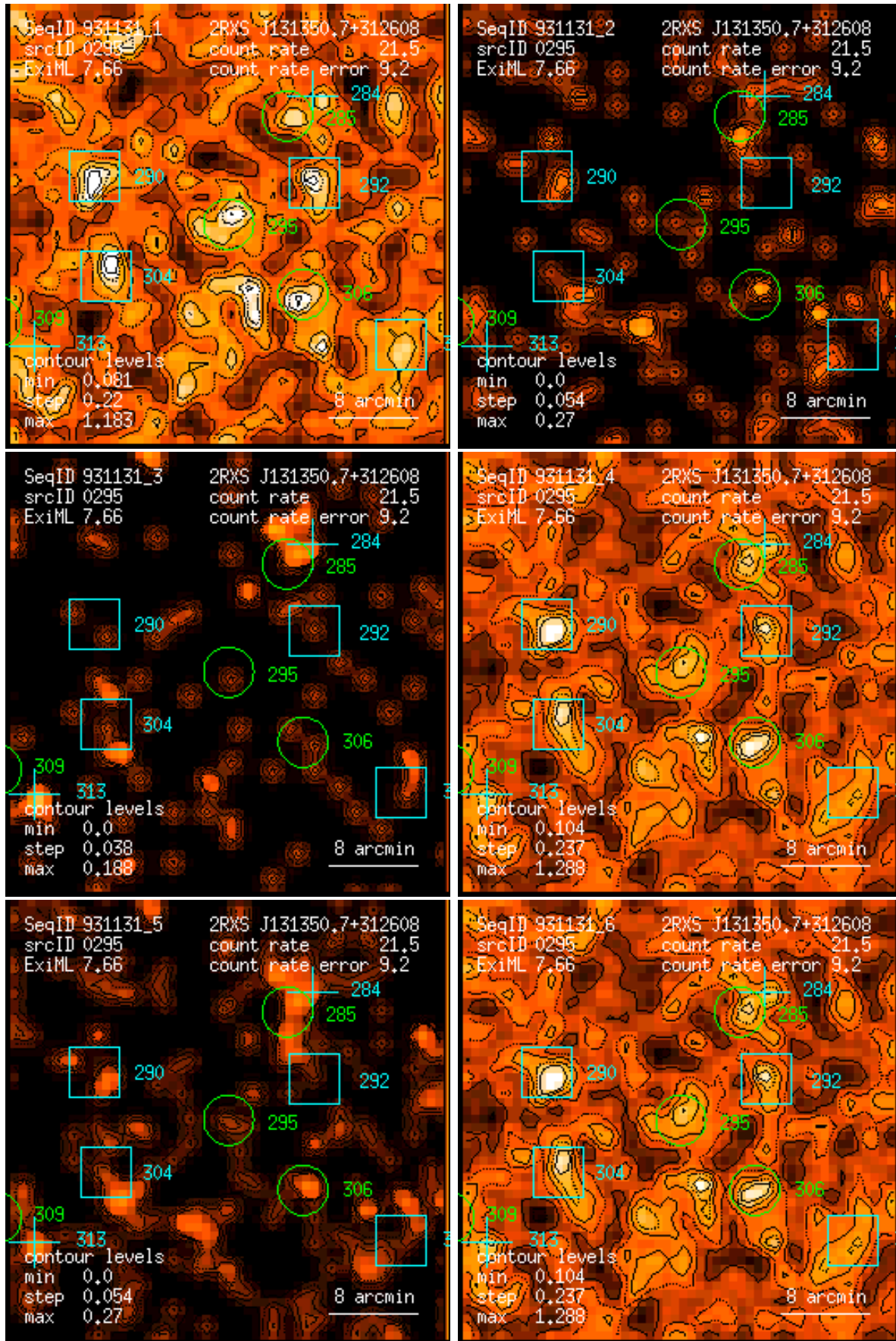
Figure 295: RASS 931131: detection 0295: band rate images, Gaussian filter: (1) PSPC channels 11 – 41, (2) 52 – 90, (3) 91 – 201, (4) 11 – 235, (5) 52 – 201, (6) 11 – 201. Broad band rates in counts/ks. Band rate contour levels in counts/ks/arcmin 2 .
