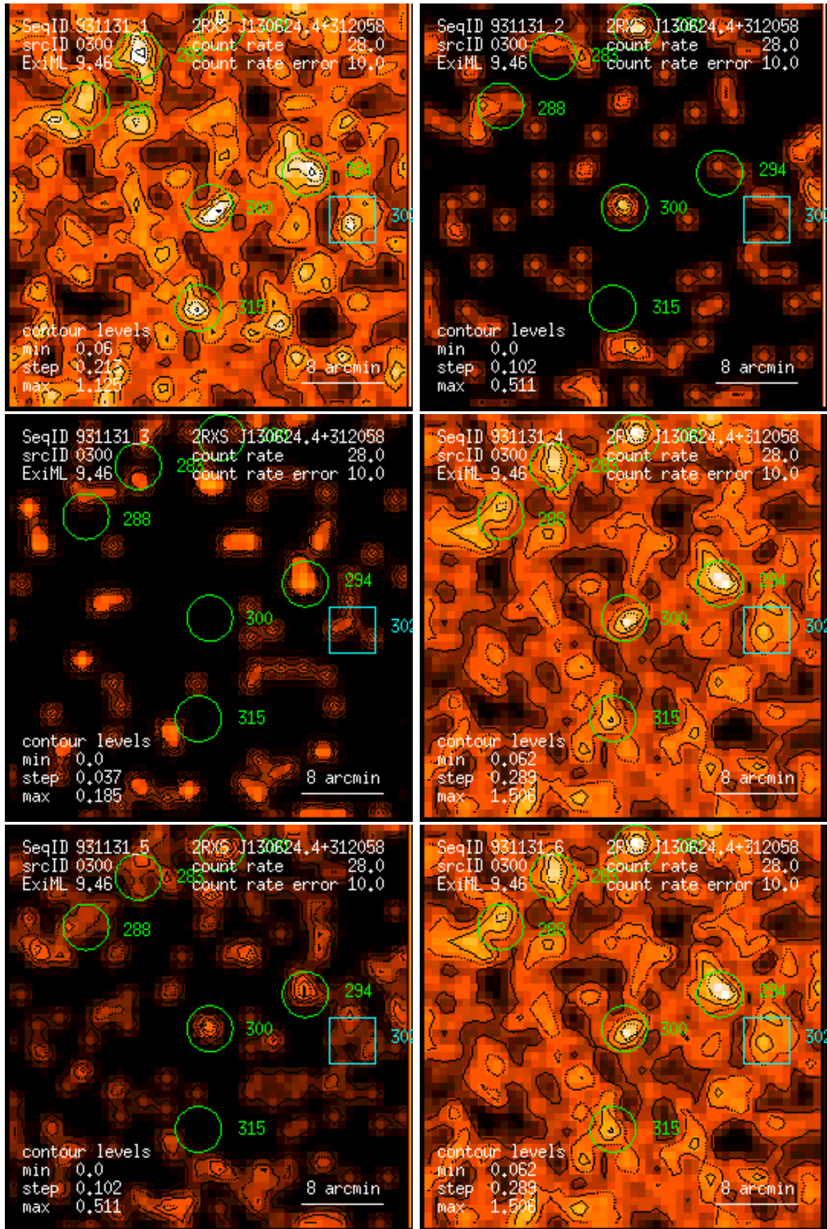
Figure 300: RASS 931131: detection 0300: band rate images, Gaussian filter: (1) PSPC channels 11 – 41, (2) 52 – 90, (3) 91 – 201, (4) 11 – 235, (5) 52 – 201, (6) 11 – 201. Broad band rates in counts/ks. Band rate contour levels in counts/ks/arcmin 2 .
