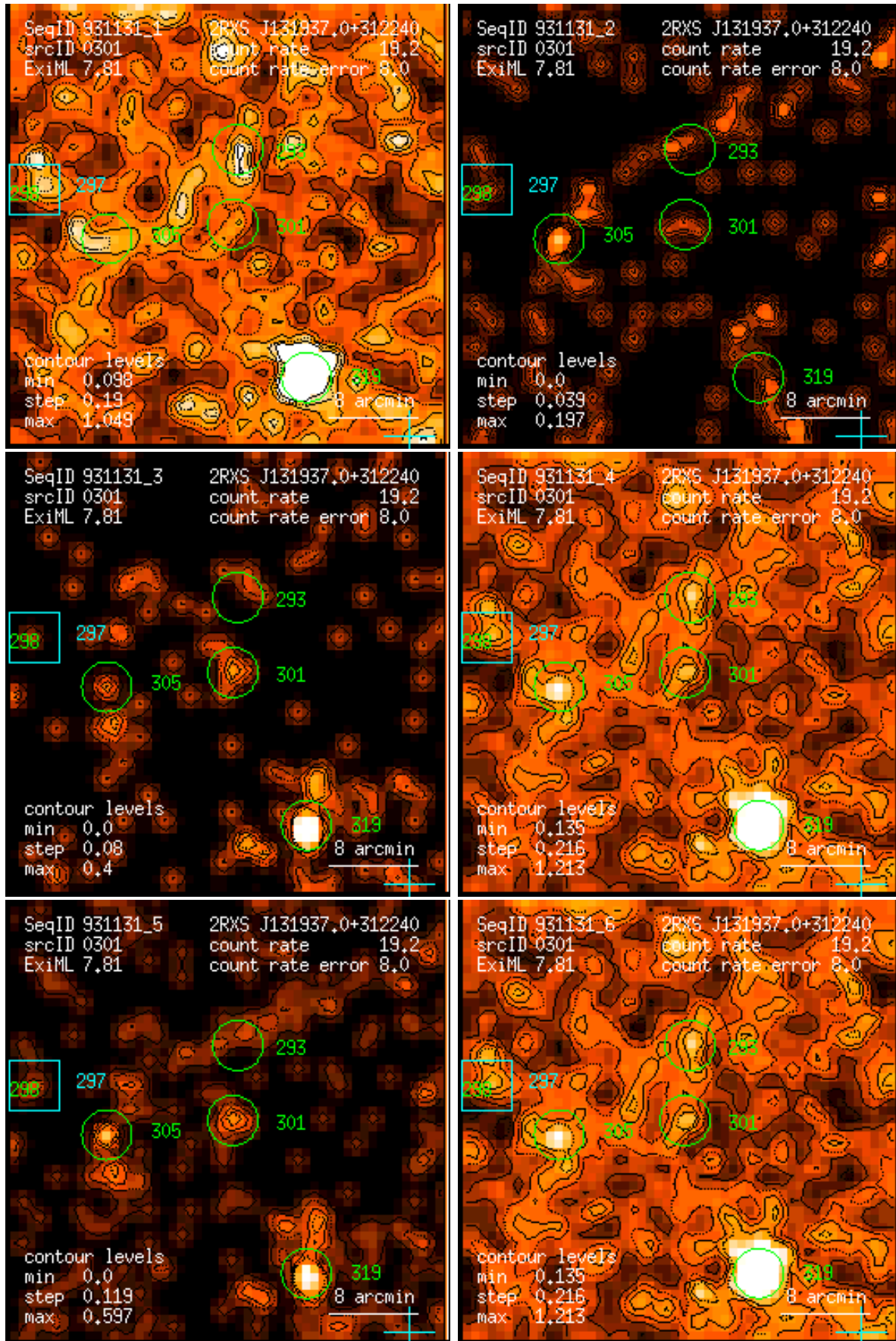
Figure 301: RASS 931131: detection 0301: band rate images, Gaussian filter: (1) PSPC channels 11 – 41, (2) 52 – 90, (3) 91 – 201, (4) 11 – 235, (5) 52 – 201, (6) 11 – 201. Broad band rates in counts/ks. Band rate contour levels in counts/ks/arcmin 2 .
