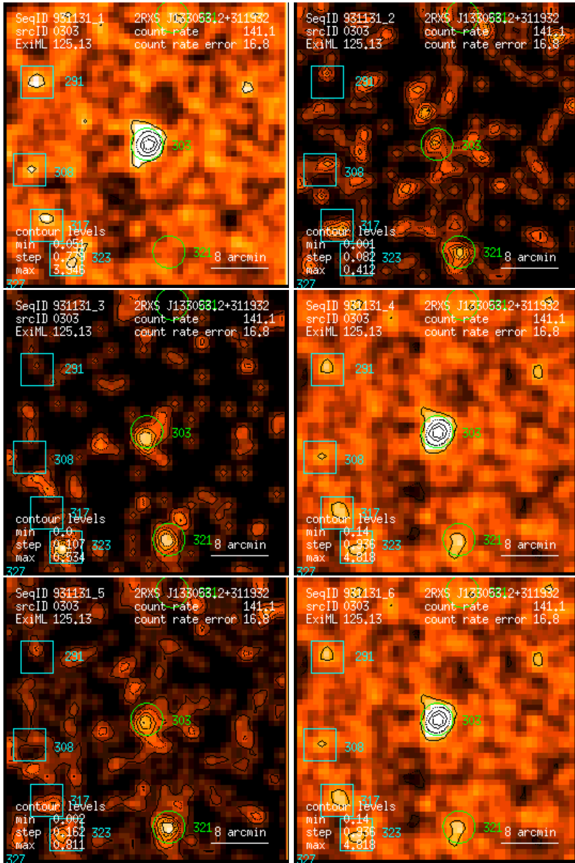
Figure 303: RASS 931131: detection 0303: band rate images, Gaussian filter: (1) PSPC channels 11 – 41, (2) 52 – 90, (3) 91 – 201, (4) 11 – 235, (5) 52 – 201, (6) 11 – 201. Broad band rates in counts/ks. Band rate contour levels in counts/ks/arcmin 2 .
