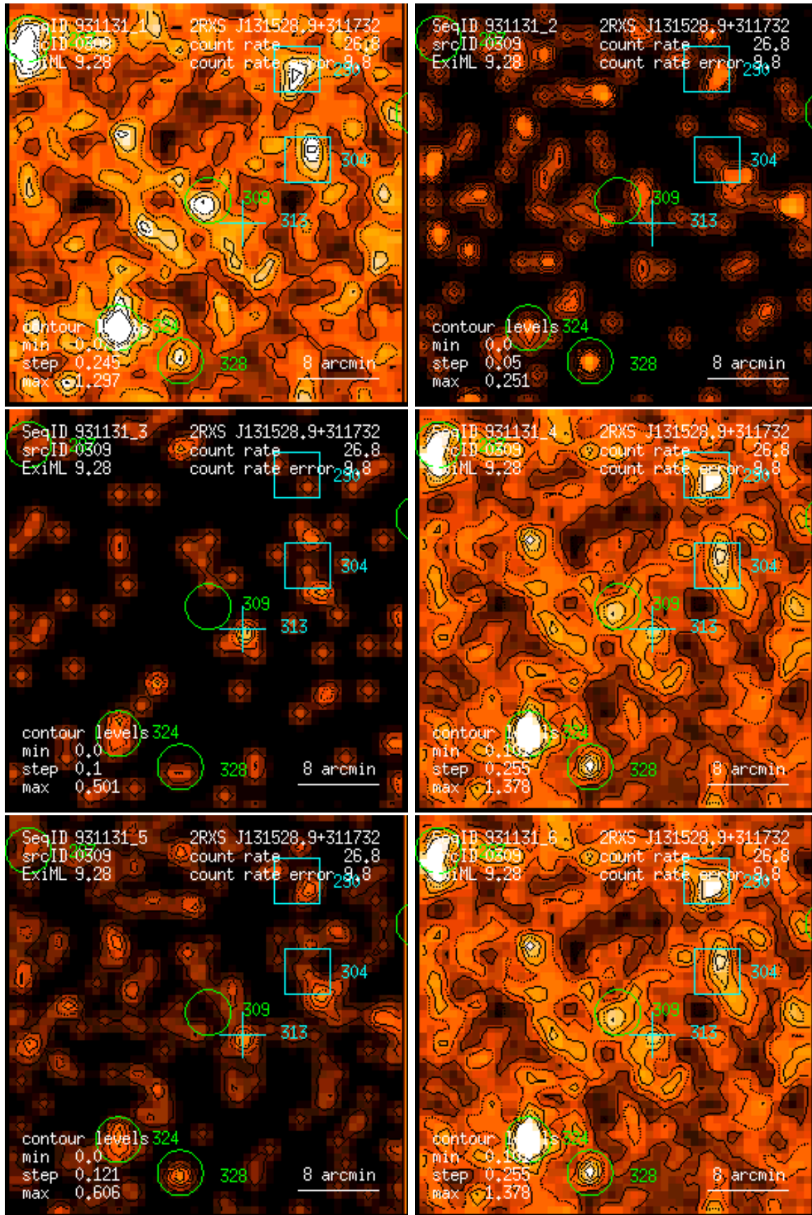
Figure 309: RASS 931131: detection 0309: band rate images, Gaussian filter: (1) PSPC channels 11 – 41, (2) 52 – 90, (3) 91 – 201, (4) 11 – 235, (5) 52 – 201, (6) 11 – 201. Broad band rates in counts/ks. Band rate contour levels in counts/ks/arcmin 2 .
